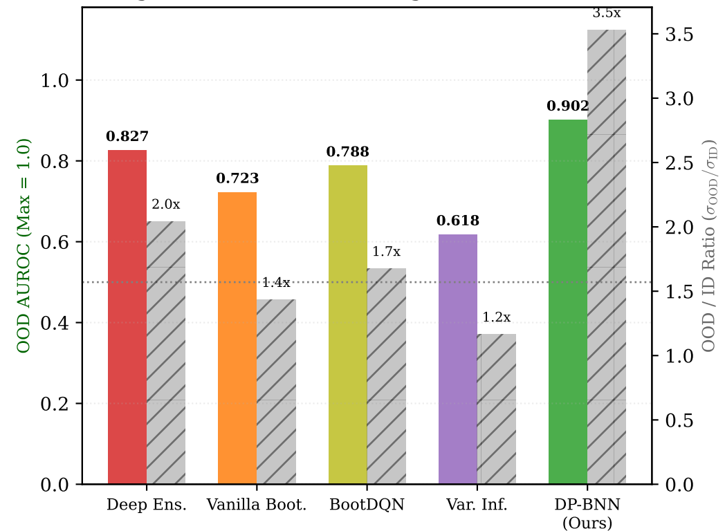
(c) Real-World UQ Summary Benchmark [Higher AUROC = Better, Higher Ratio = Better]
