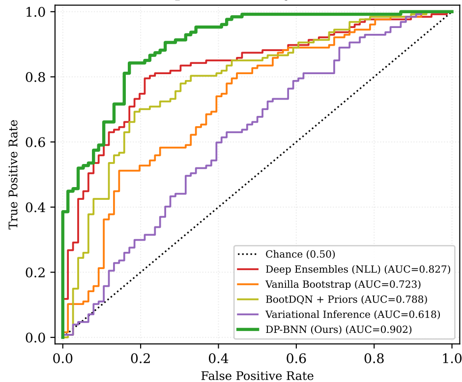
(b) OOD Detection ROC Curves [Unseen Spatial Territory Discrimination]
