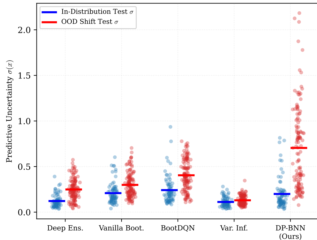
(a) Epistemic Uncertainty Under Covariate Shift [UCI Boston Housing: D = 13 , Shift along DIS]
