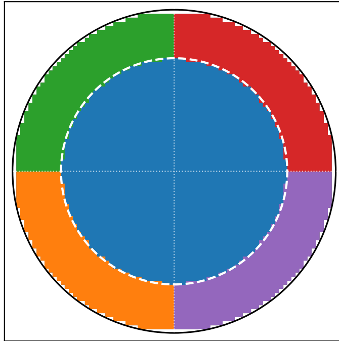
(a) Ground Truth Optimal Policy (Hub=Arm 0, Rim=Jackpot Arms 1-4)
