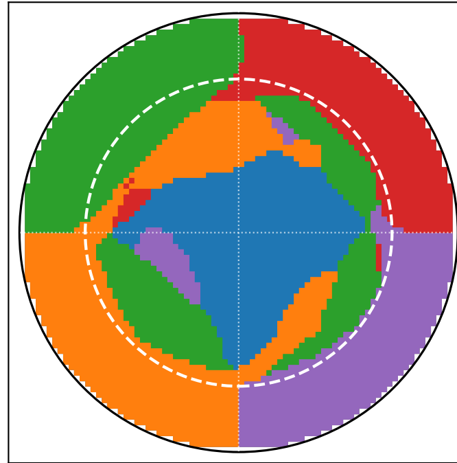
(b) Deep Ensembles Policy (Trapped in Arm 0; Misses Jackpots)
