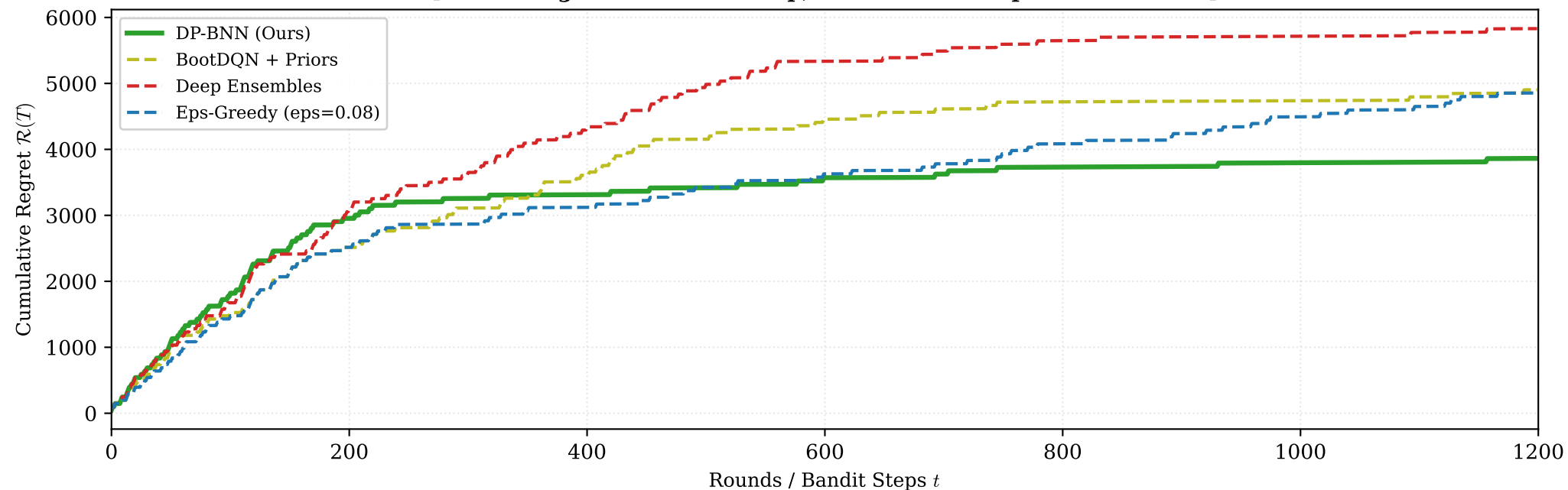
(d) Cumulative Regret over Time (Lower is Better) [Linear Regret = Stuck in Trap, Sub-Linear = Exploration Solved]
