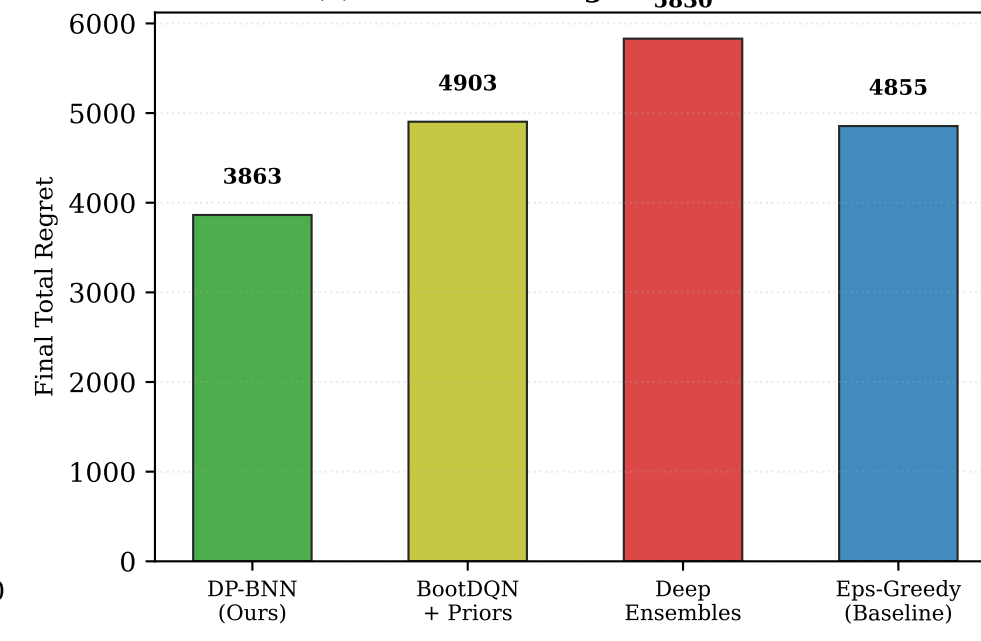
(e) Final Total Regret Benchmark
