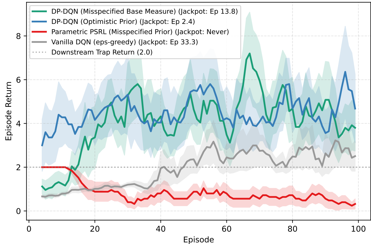
(b) Per-Episode Return (5-step avg)
