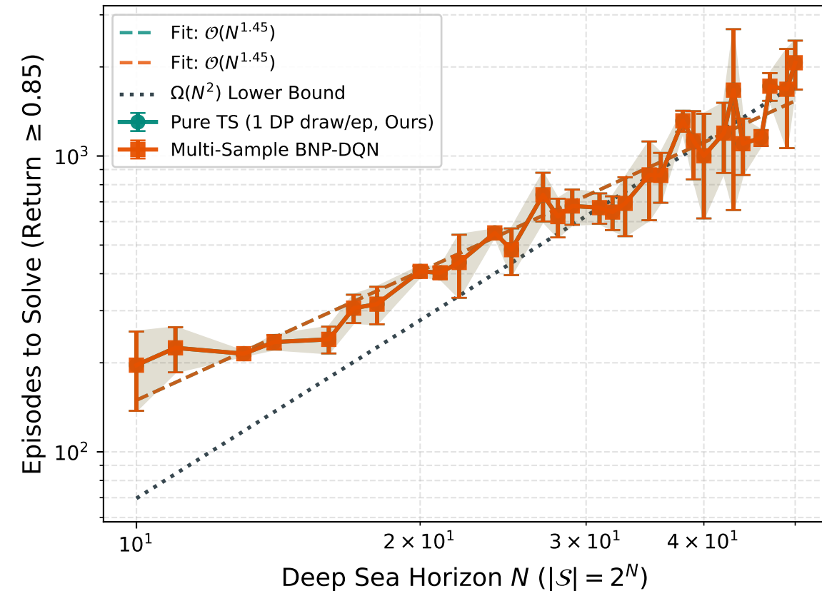
(a) Sample Complexity Scaling vs. Bound
