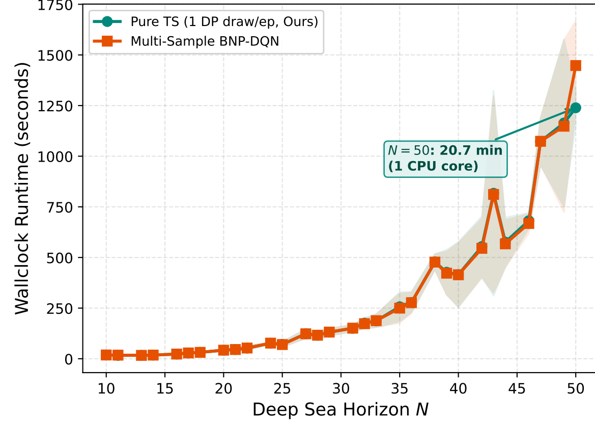
(c) Single-Core CPU Runtime Scaling
