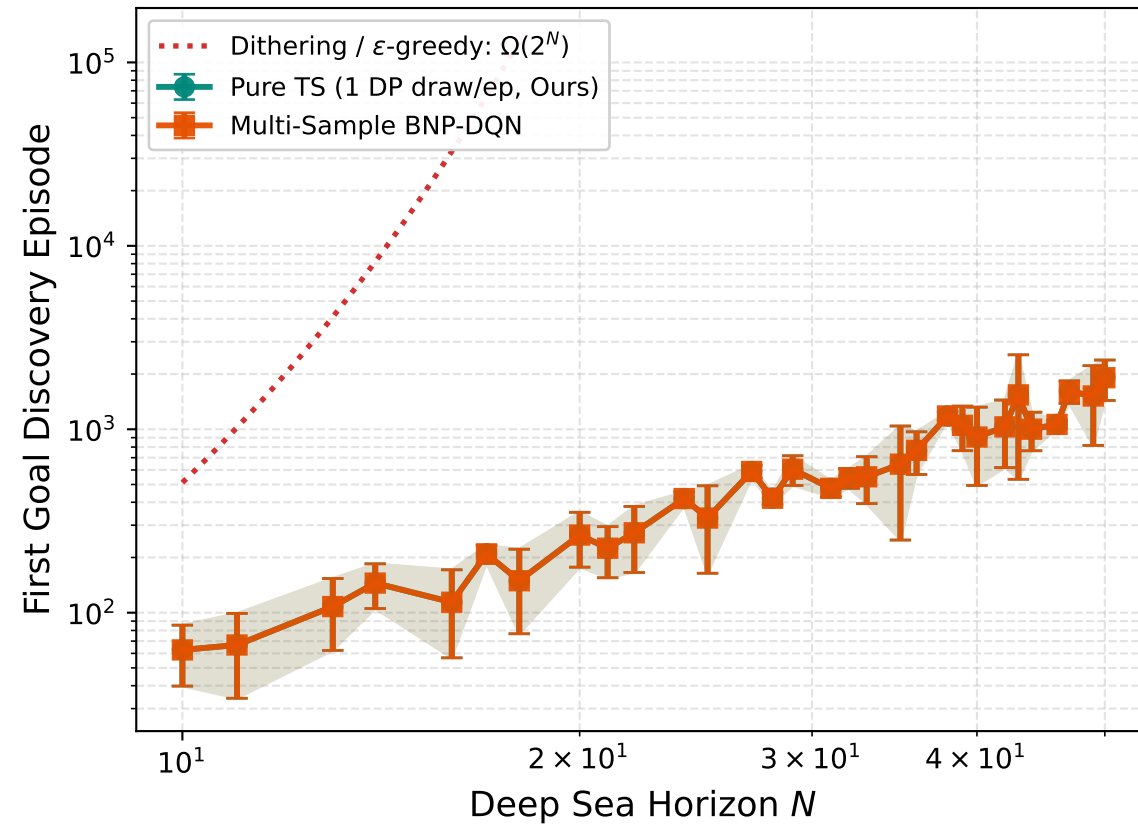
(b) Goal Discovery Horizon ( T_{\text{disc}} )
