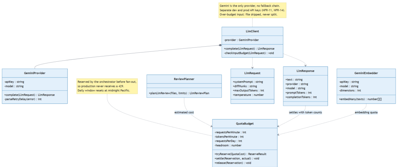
Figure 4.3 LLM client class diagram
