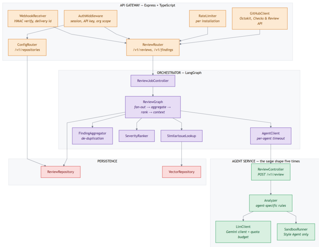
Figure 2.2 Component diagram
