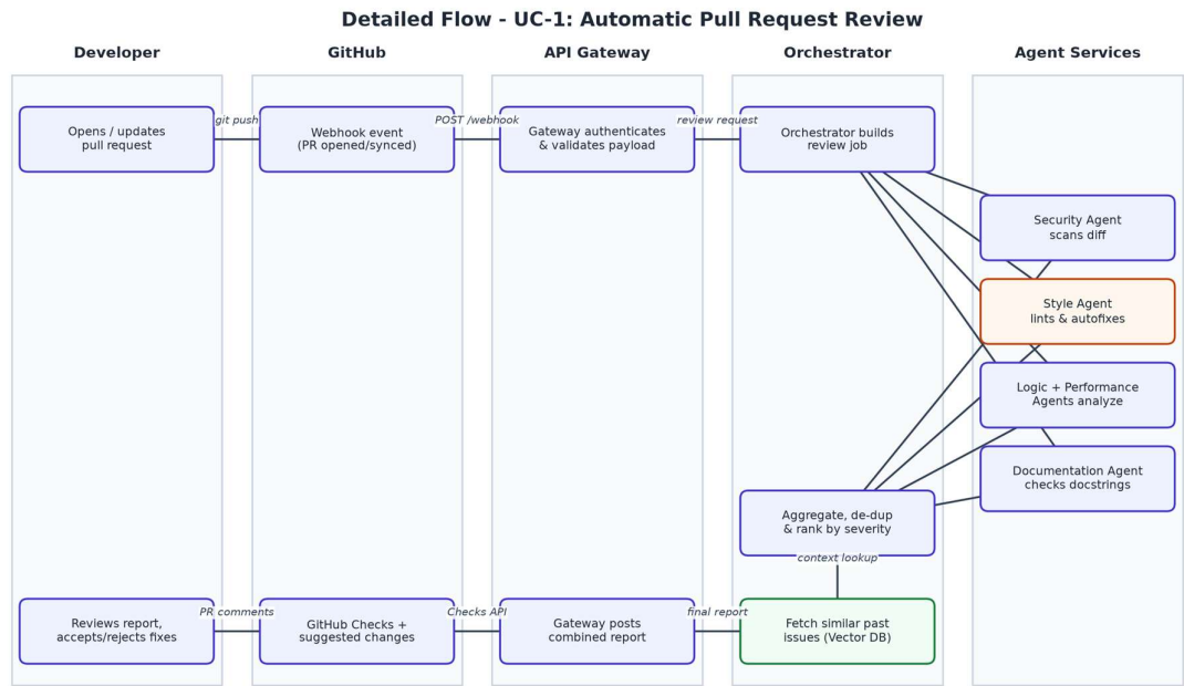
Figure 5.2 — Detailed swimlane flow for UC-1: Automatic Pull Request Review
