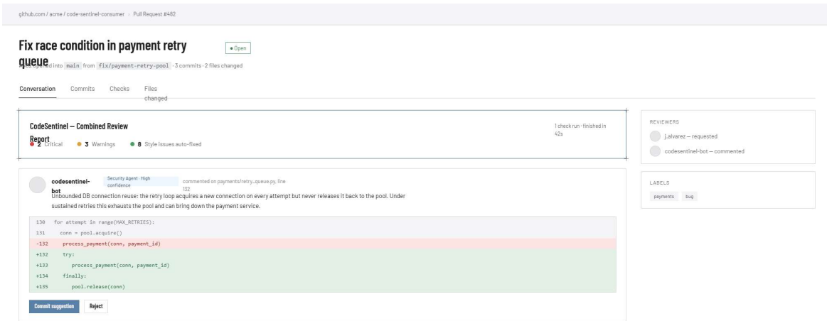
Figure 7.1 — GitHub PR inline suggested-change comment (initial draft)
