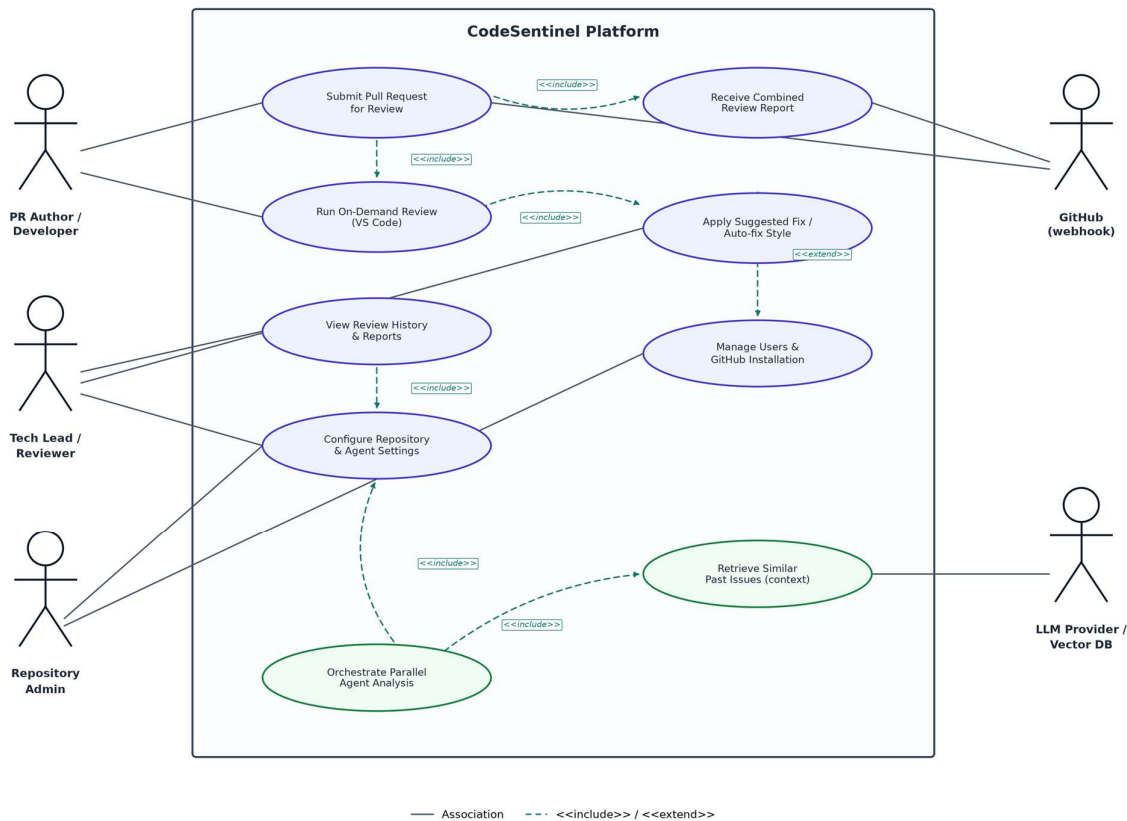
Figure 5.1 — Primary use case diagram for the Code-Sentinel platform
