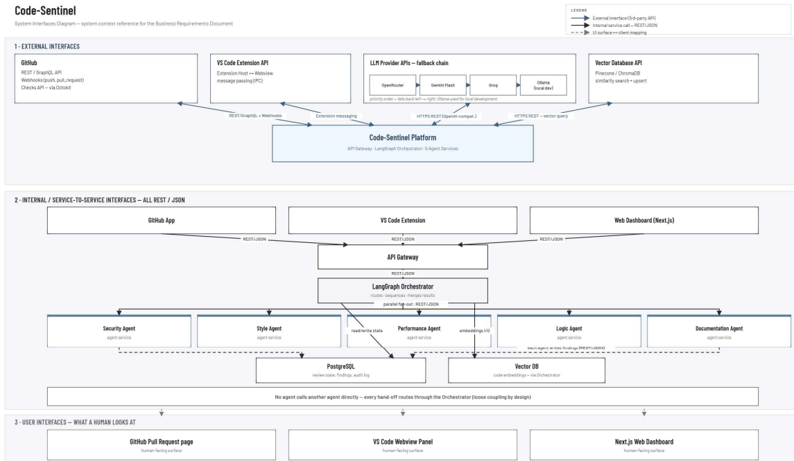
Figure 6.1 — Code-Sentinel system interfaces diagram
