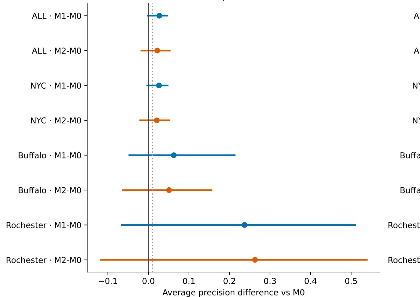
Buffered spatial holdouts
