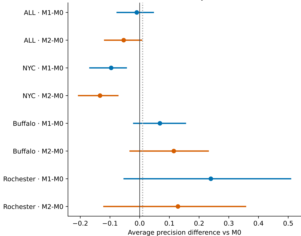
Leave one city out
