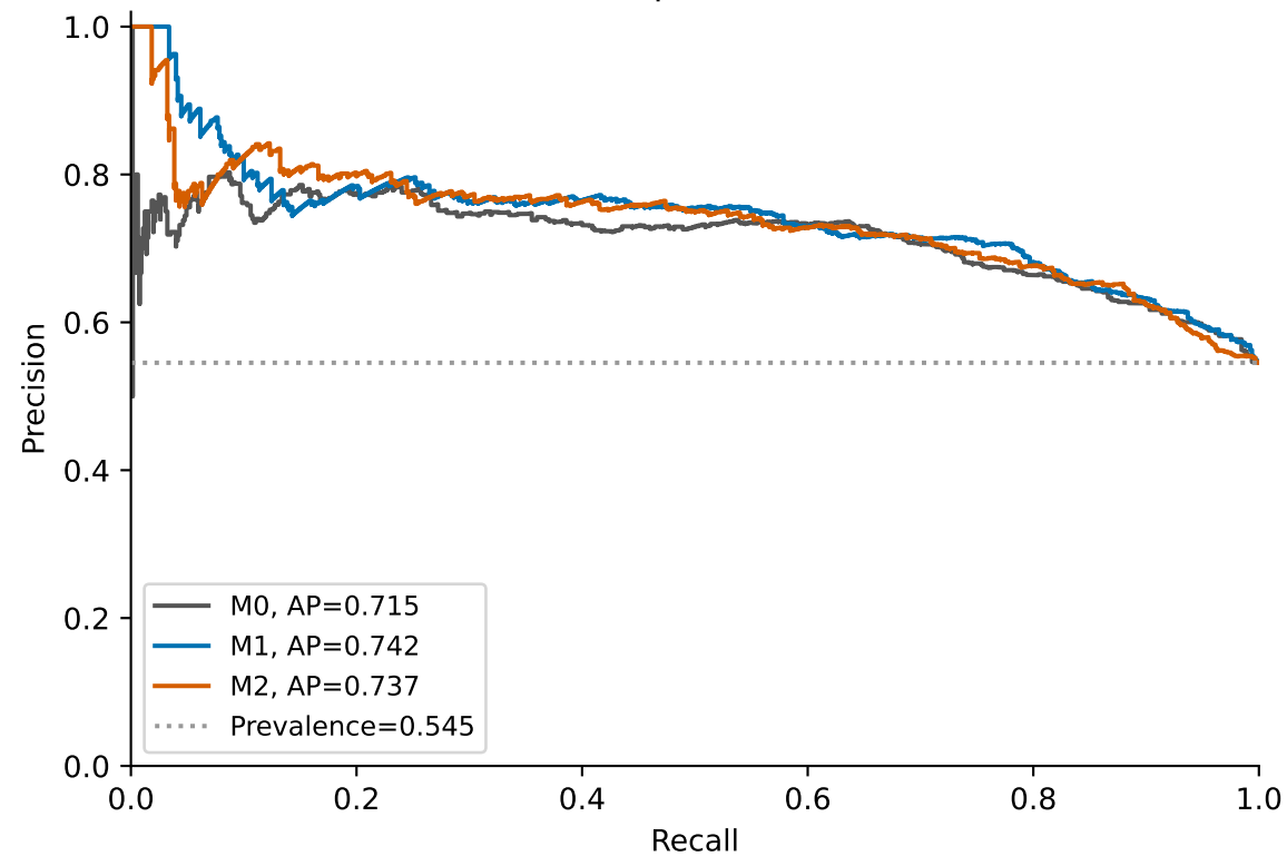
Buffered spatial holdouts
