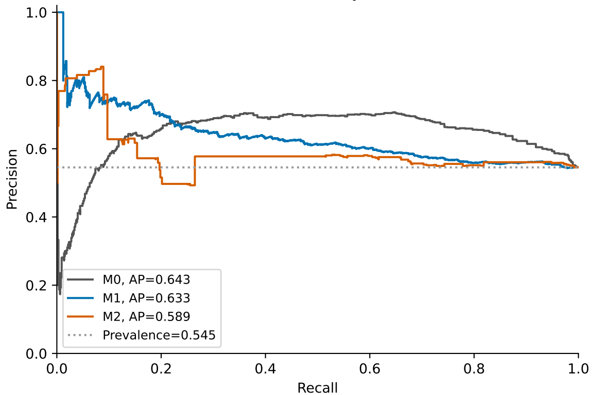
Leave one city out
