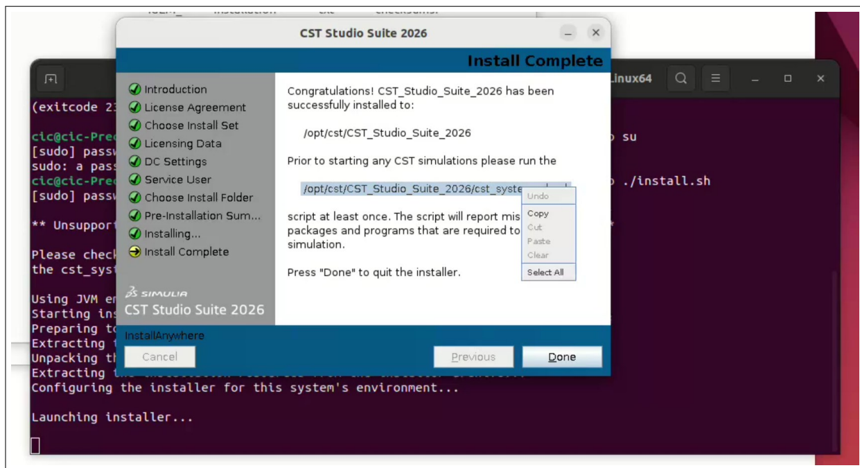
Figure 17: Install completion page showing the default installation path and the system check command.
