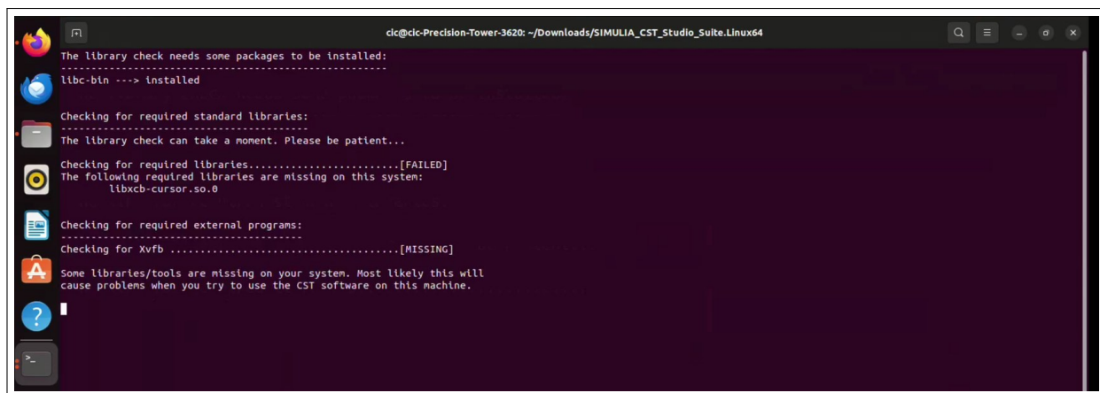
Figure 21: System check output reporting missing libraries and tools.
