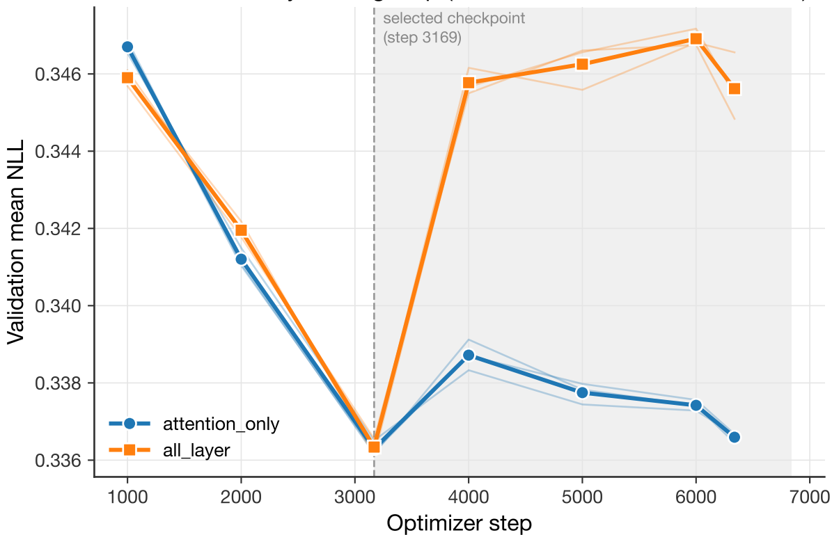
Validation NLL by training step (main-001, both LoRA conditions)
