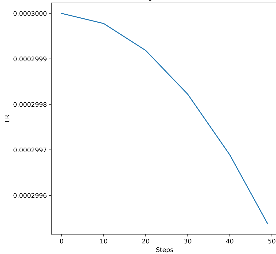
Learning Rate Schedule
