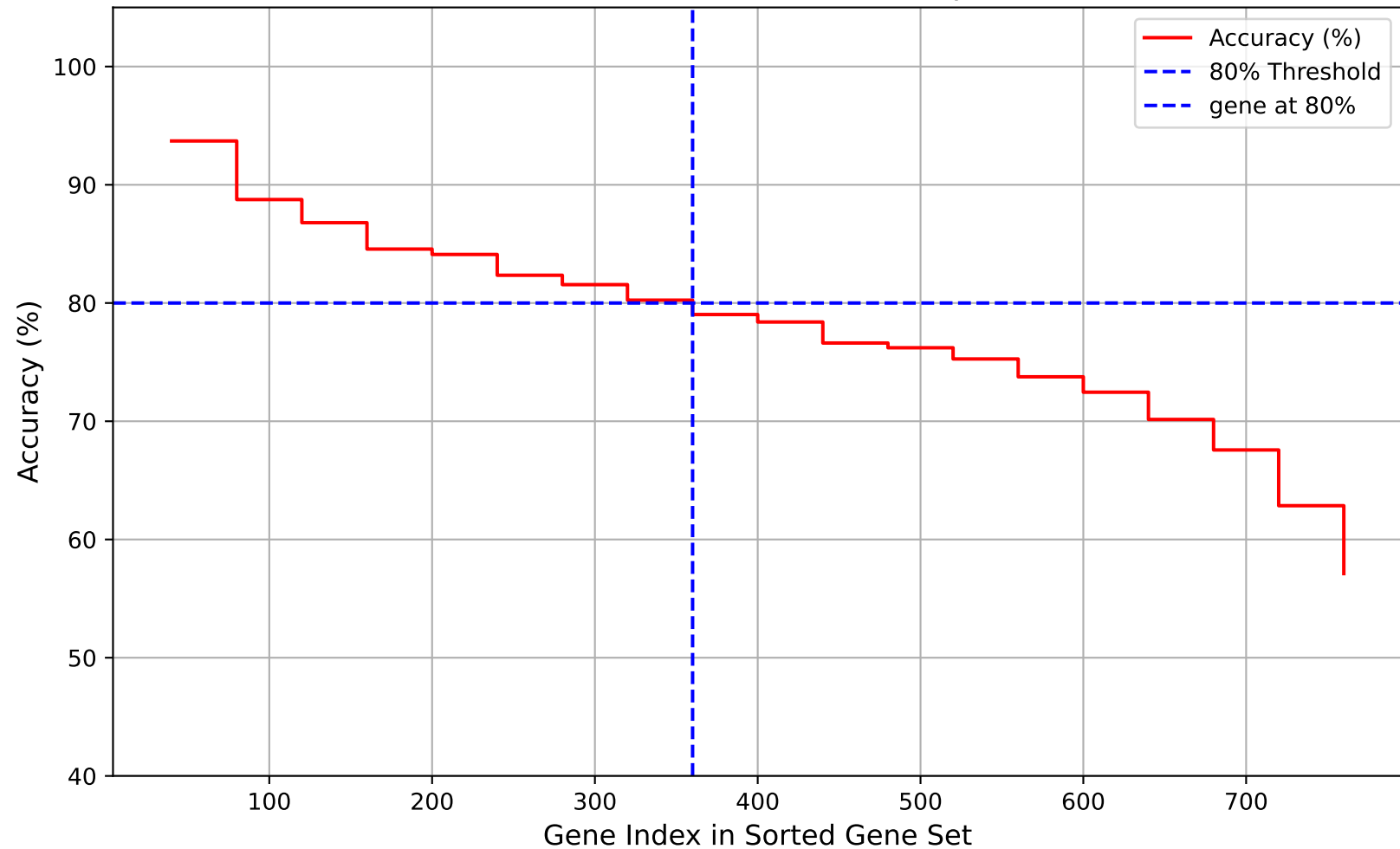
(GSE9844)Random Forest Step Plot
