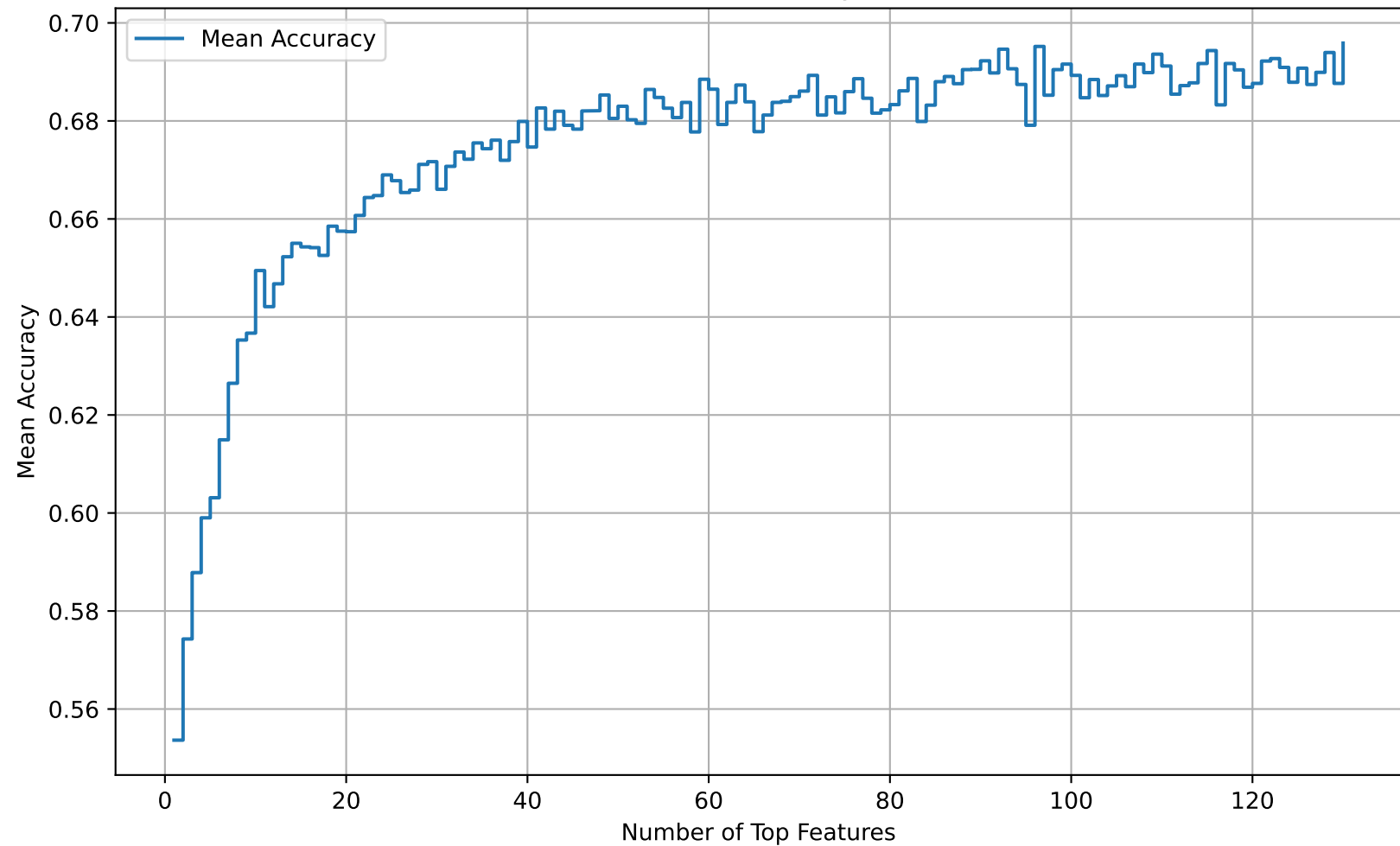
Cumulative Mean Accuracy Across Folds
