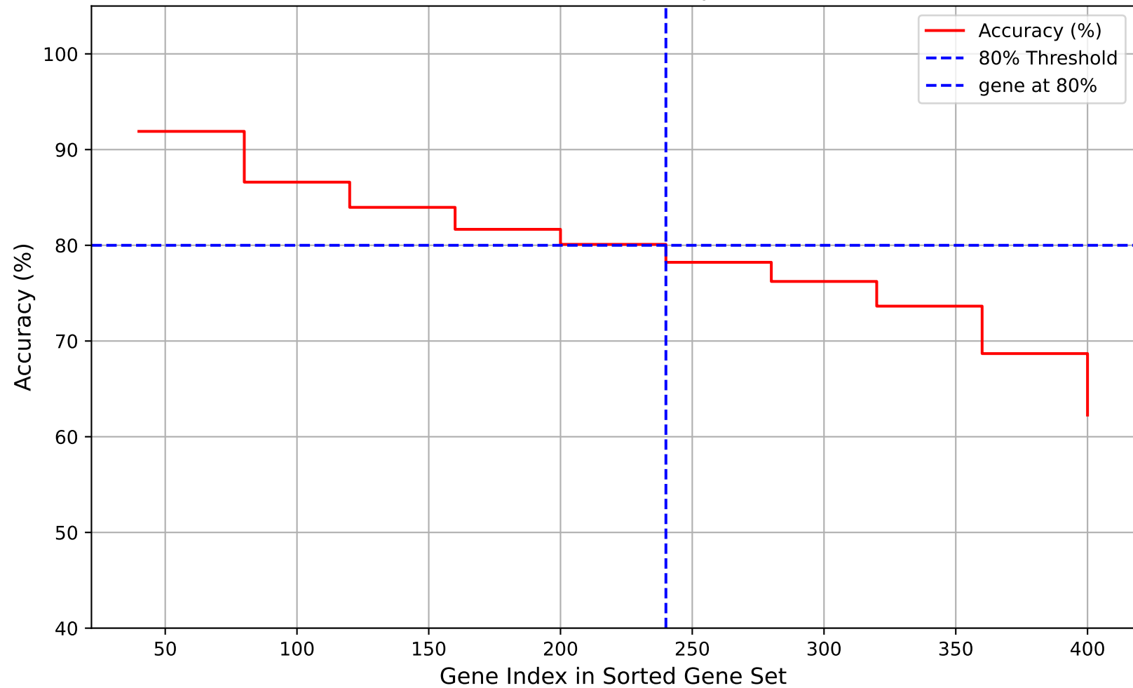
(GSE9844)SVM Step Plot
