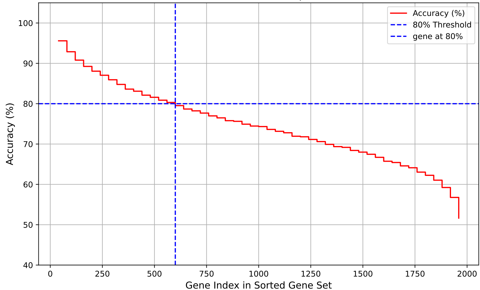
(GSE34105)KNN Step Plot
