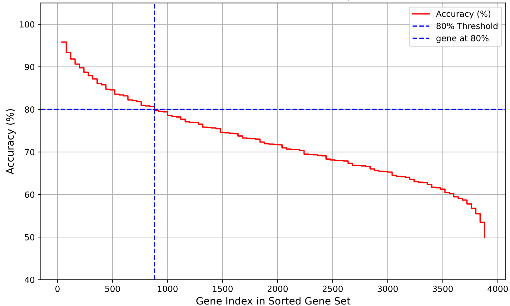
(GSE34105)Random Forest Step Plot
