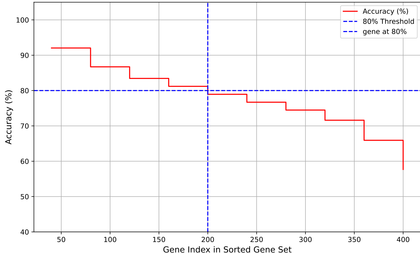
(GSE9844)KNN Step Plot
