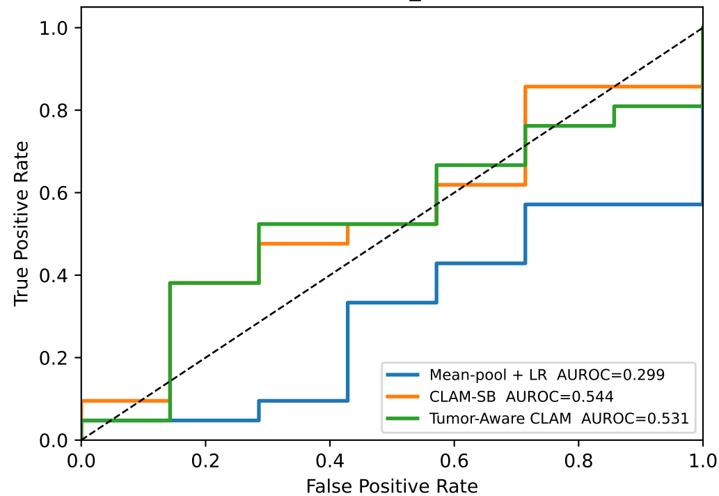
ROC — ER_status
