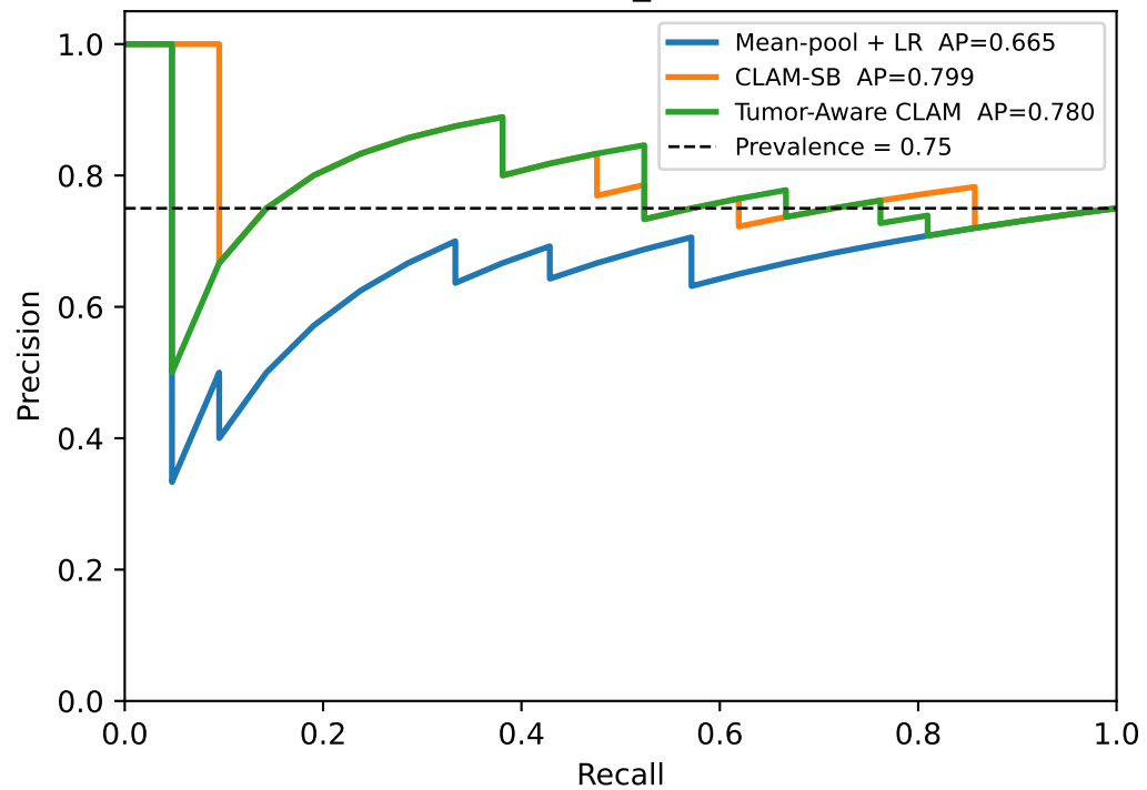
PR — ER_status
