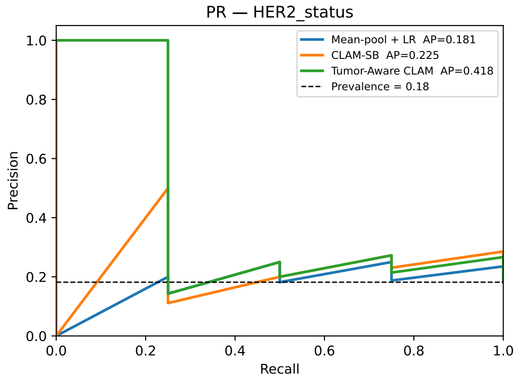
Ablation — HER2_status (test set)
