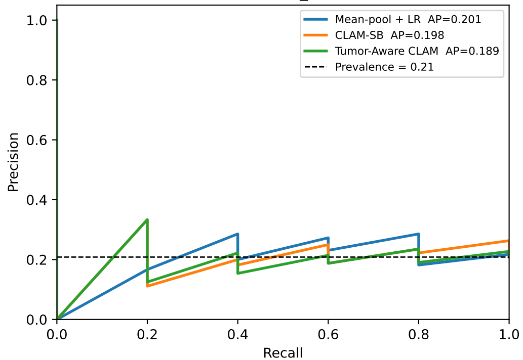
PR — HER2_status
