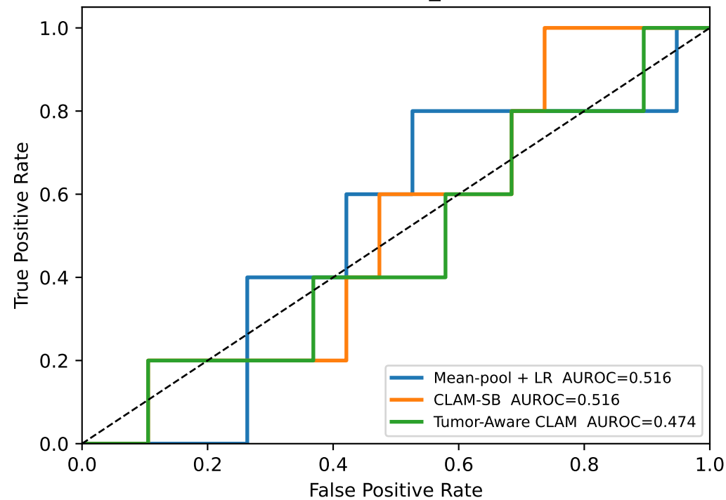
ROC — HER2_status
