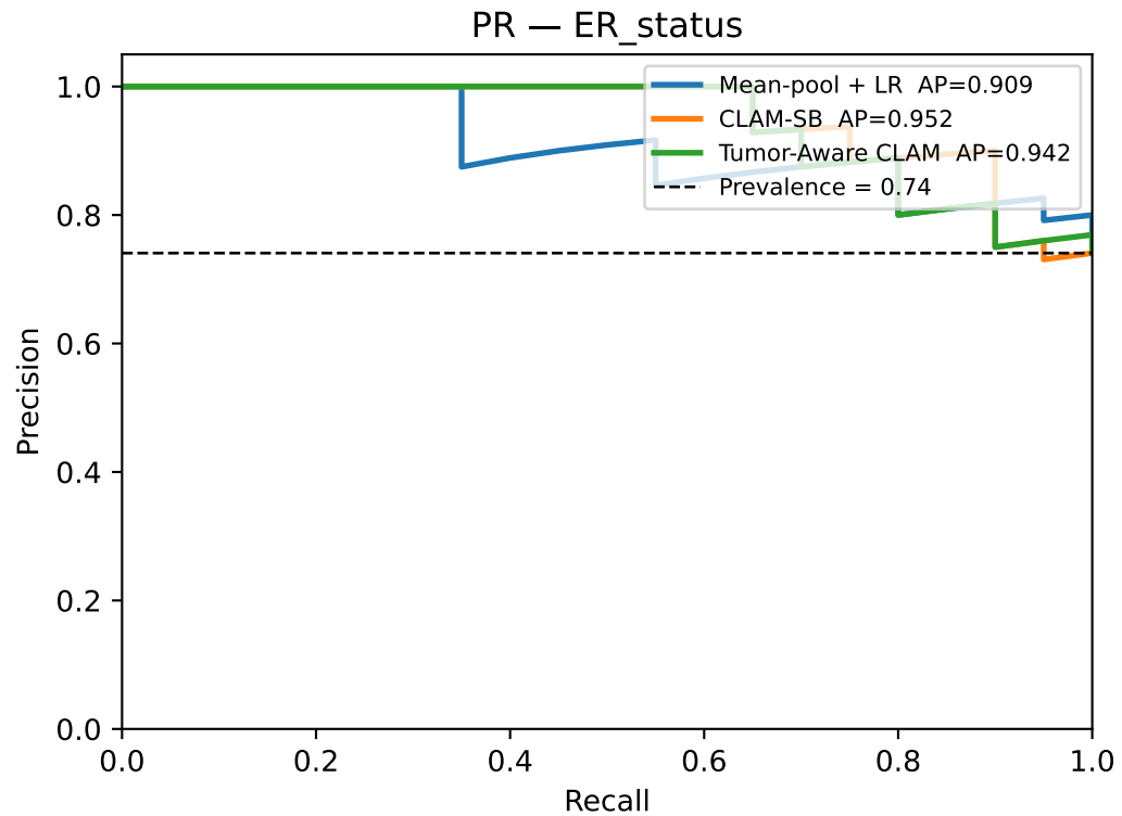
Ablation — ER_status (val set)
