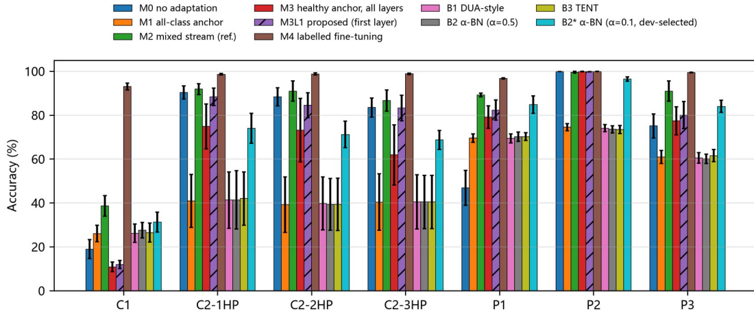
Figure S2. Accuracy of all methods on the seven target domains (mean \pm std over 5 seeds); the data are those of Table 5 of the paper.
