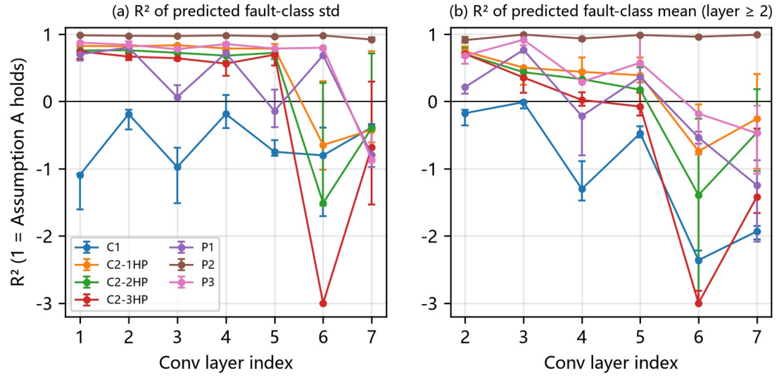
Figure S5. Test of Assumption A: R^2 of the predicted fault-class standard deviation (a) and mean (b, from layer 2) per layer (median of 5 seeds; bars show the interquartile range; values below -3 are drawn at the lower bound).
