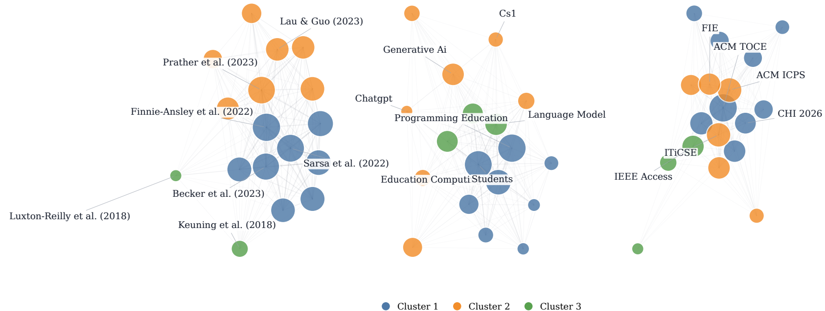
(a) Co-citation
