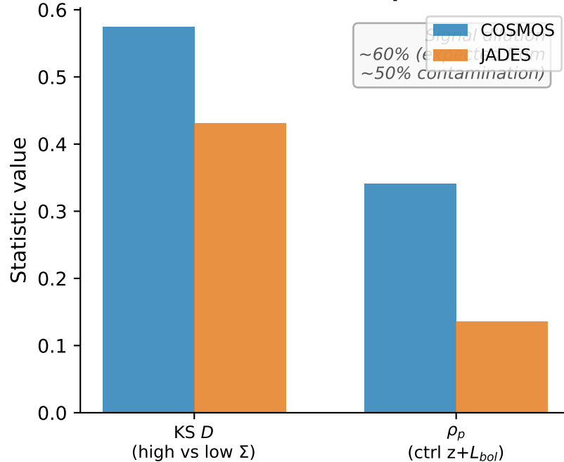
(b) Controlled Comparison
