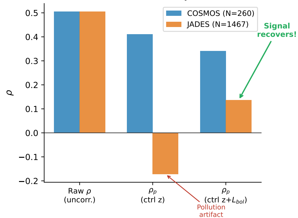
(a) Correlation Comparison
