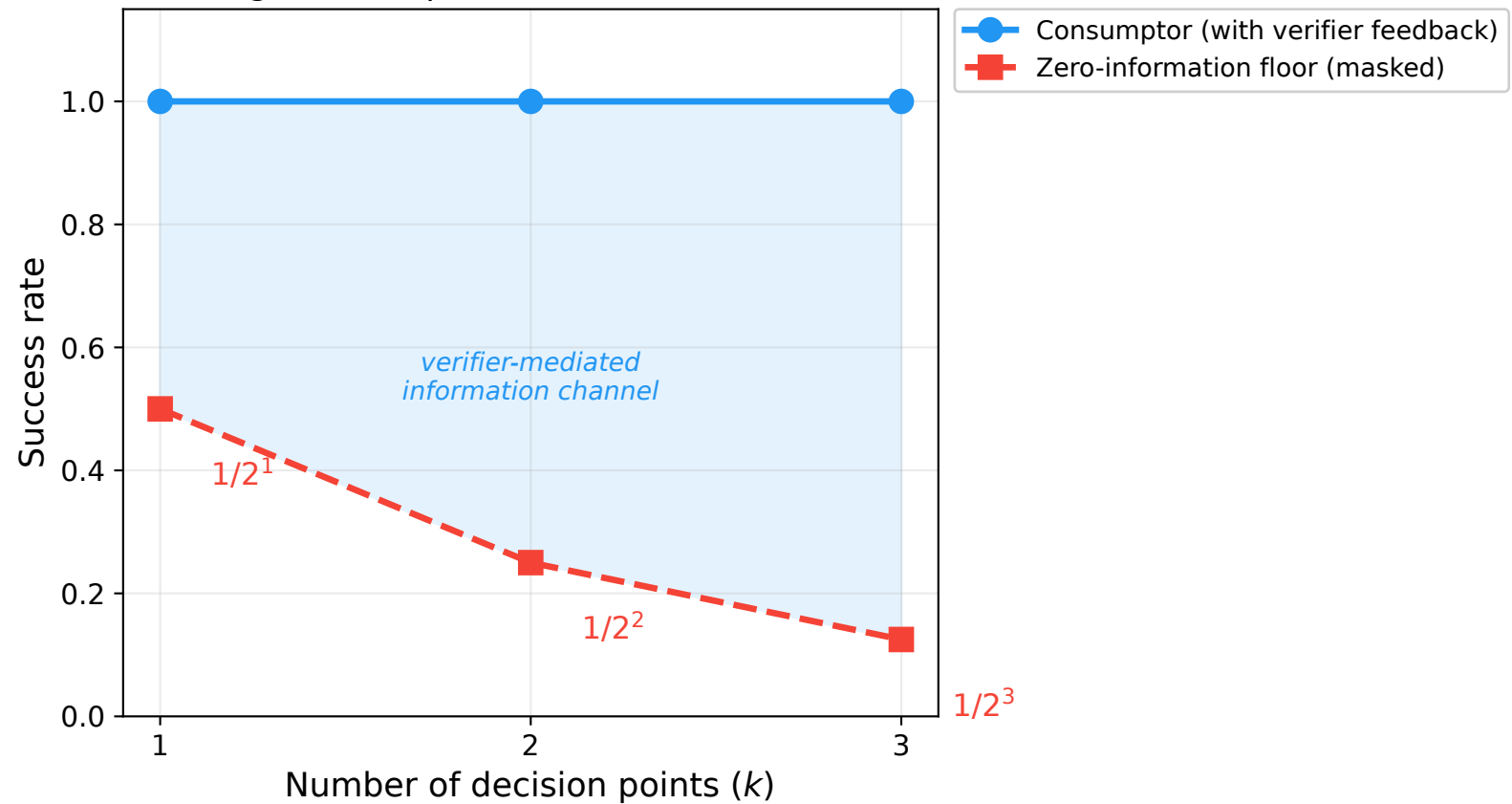
Scaling: Consumtor vs zero-information floor
