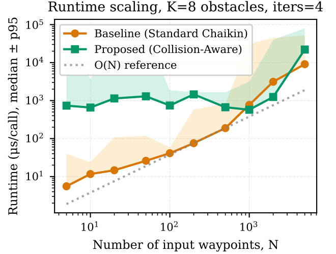
Figure 1: Runtime vs. input size, K=8 obstacles, 20 trials per point. Bands show median to 95th percentile. Dotted line is the O(N) reference, anchored at N=200 .
