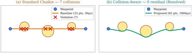
Figure 7: Pillars scenario. Baseline crosses three discs; proposed detours around all three.
