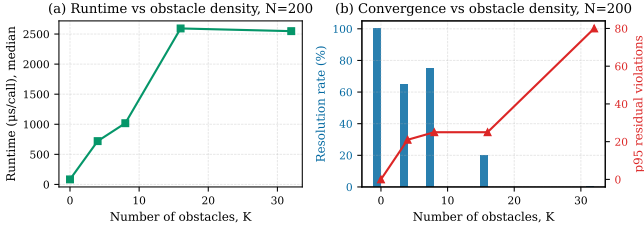
Figure 3: Effect of obstacle count, N=200 . (a) Runtime grows roughly linearly with K , then saturates when the safety deadline fires. (b) Resolution rate (left bars) collapses from 100% at K=0 to 0% at K=32 . The red line is the 95th-percentile unfixed-collision count.
