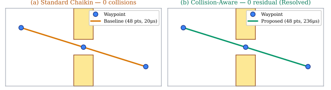
Figure 8: Narrow-gap scenario. Waypoints already go through the gap; both methods produce the same answer with no collisions.
