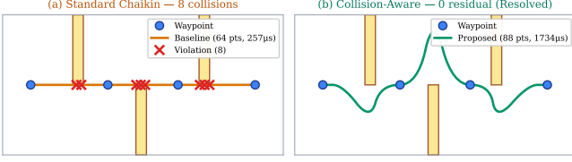
Figure 6: Corridor scenario. Baseline cuts through three wall fingers (red \times marks); proposed method weaves around them.
