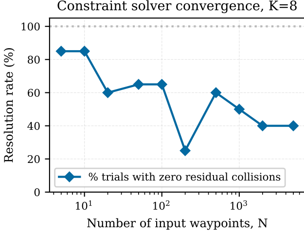
Figure 2: Resolution rate vs. input size. The proposed method does not always succeed; performance degrades when waypoints force the path through obstacle clusters.
