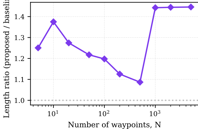
(b) Path-length overhead from detours
