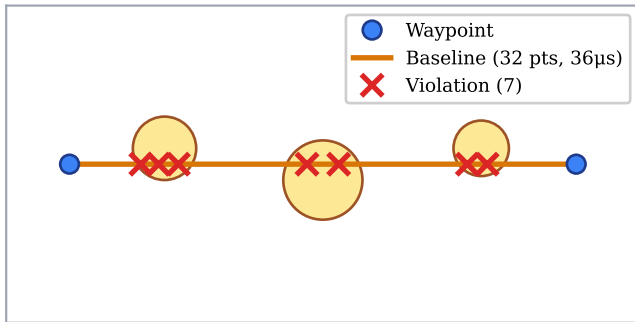
(a) Standard Chaikin — 7 collisions
