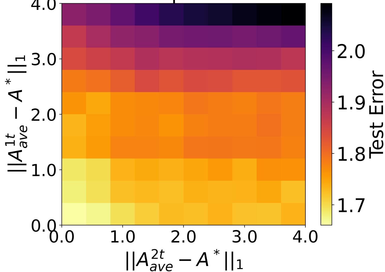
2D Heatmap of Test Error
