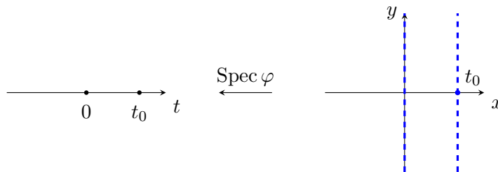
Figure 2: \text{Spec } \varphi and its fibers
