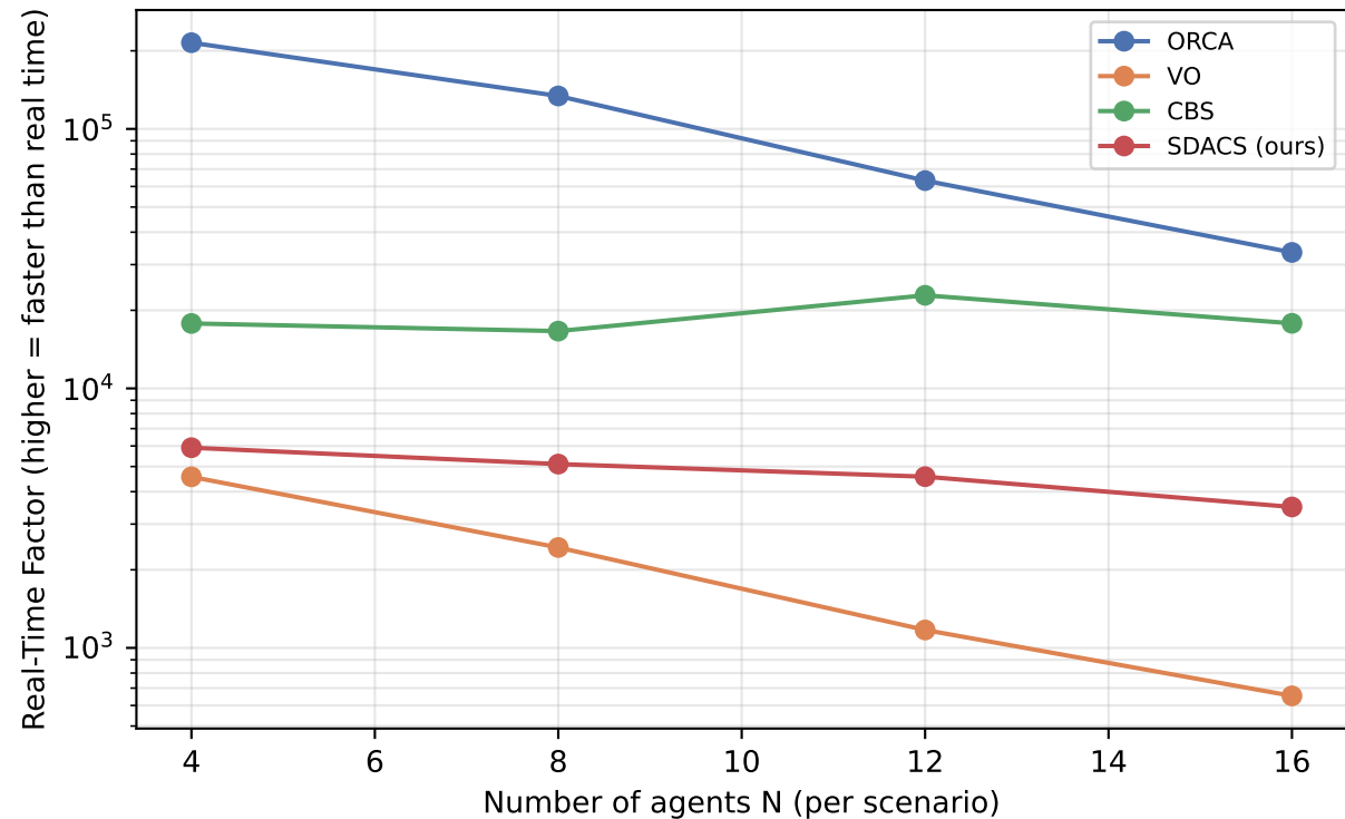
Fig. 4 Runtime scaling — RTF vs. N (RTF > 1 means the simulator runs faster than real time)
