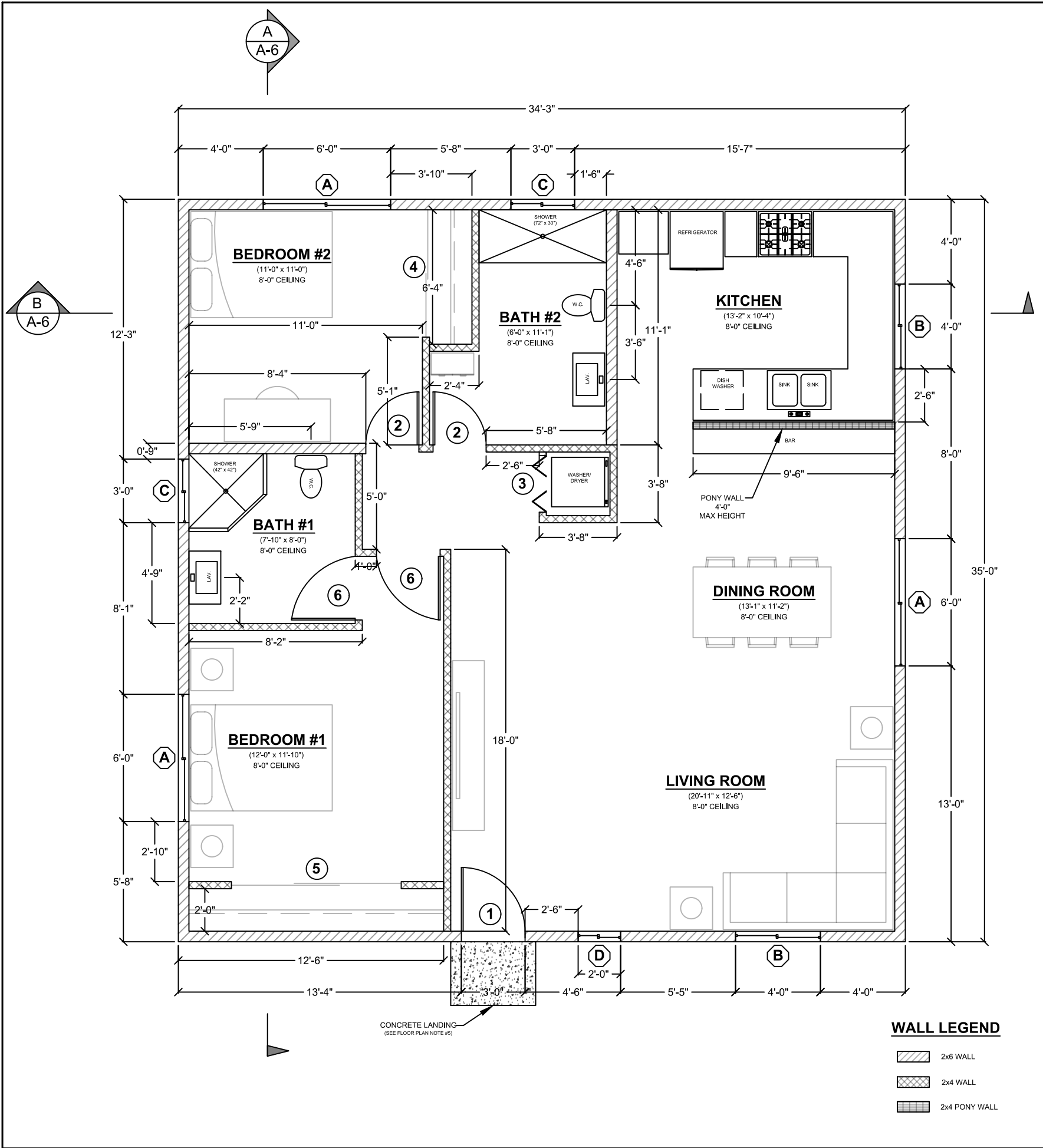
FLOOR PLAN 3/16" = 1'-0"
