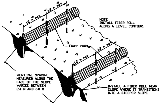
TYPICAL FIBER ROLL INSTALLATION NO SCALE
