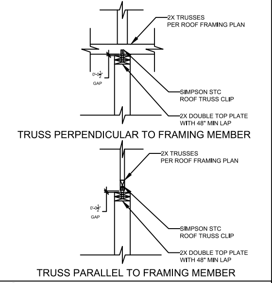
3 NON-BEARING WALL
