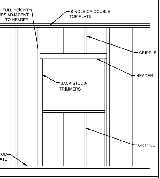
5 TYPICAL FRAMING AT OPENING
