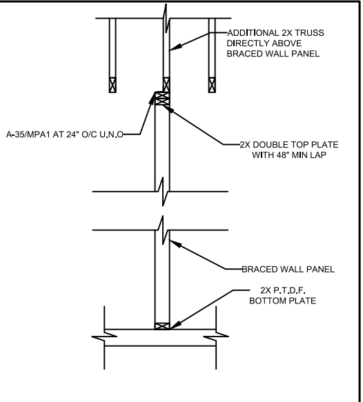
4 BRACED WALL PANEL PARALLEL TO CEILING FRAMING
