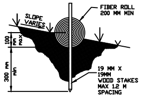
ENTRENCHMENT DETAIL NO SCALE
