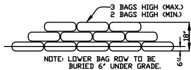
GRAVEL BAG CHECK DAM NO SCALE
