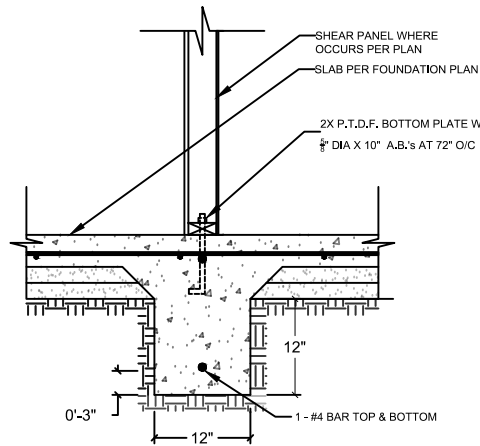
2 INTERIOR FOOTING
