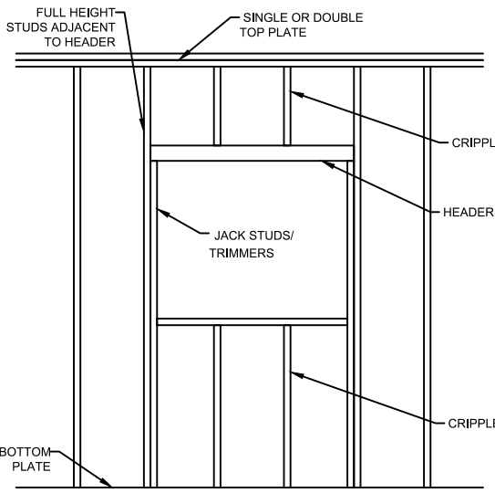
6 TYPICAL FRAMING AT OPENING
