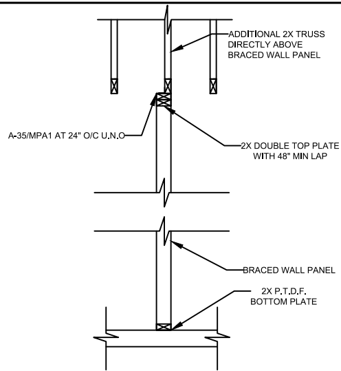
4 BRACED WALL PANEL PARALLEL TO CEILING FRAMING
