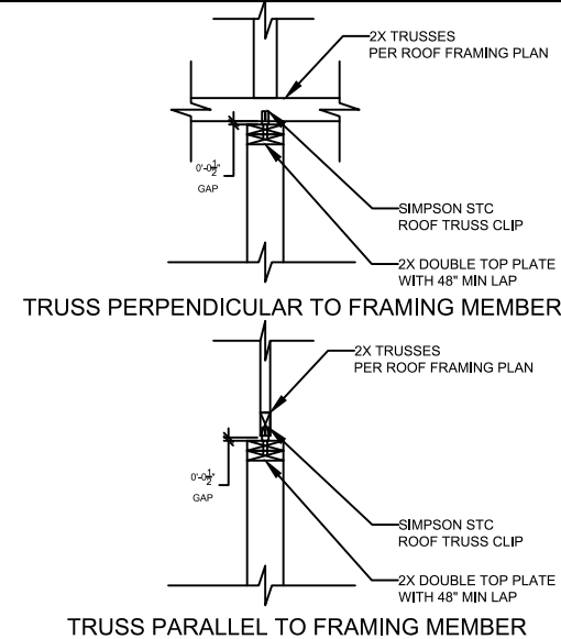
3 NON-BEARING WALL
