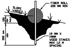
ENTRENCHMENT DETAIL NO SCALE
