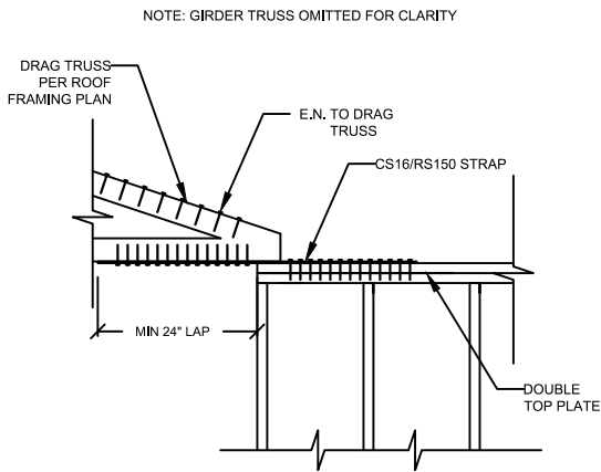
5 DRAG TRUSS CONNECTION
