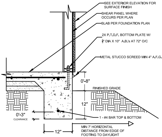
1 EXTERIOR FOOTING
