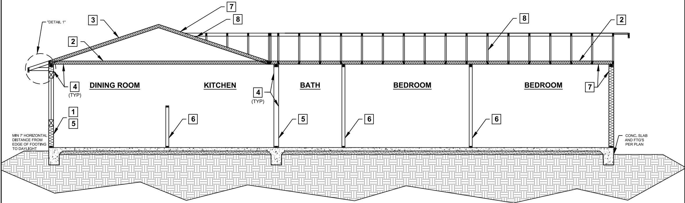
SECTION B-B
