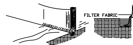
SILT FENCE NO SCALE
