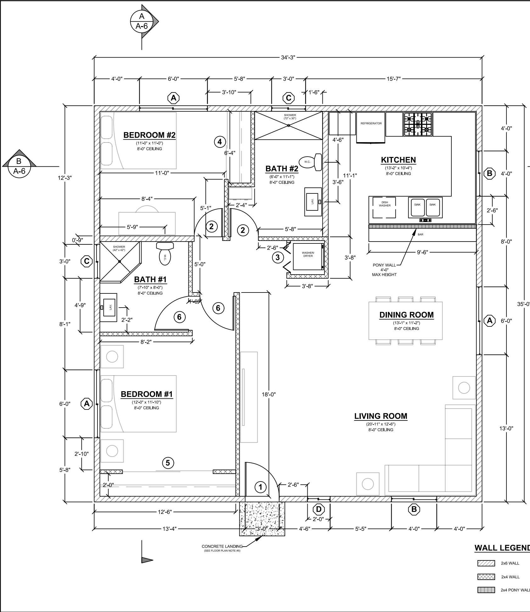
FLOOR PLAN 3/16" = 1'-0"
