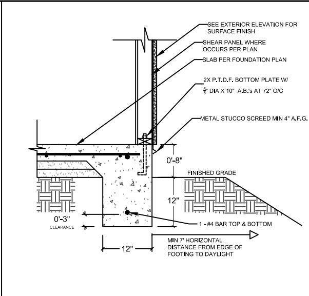
1 EXTERIOR FOOTING
