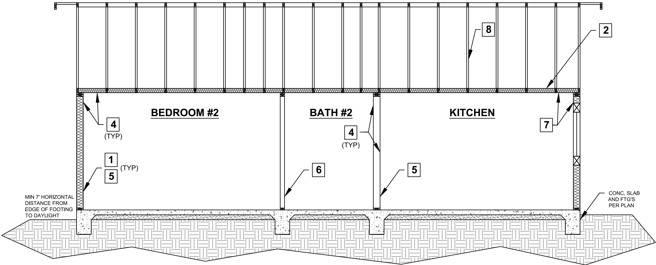
SECTION B-B
