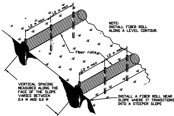
TYPICAL FIBER ROLL INSTALLATION NO SCALE
