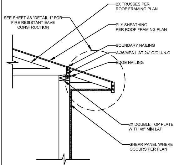
1 EAVE (SHEAR TRANSFER)
