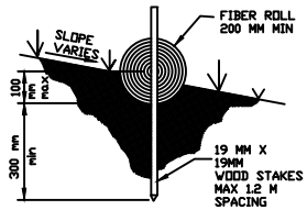
ENTRENCHMENT DETAIL NO SCALE
