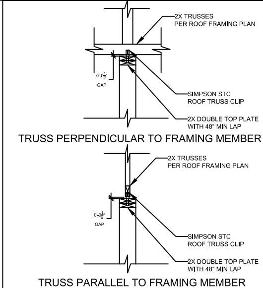
3 NON-BEARING WALL
