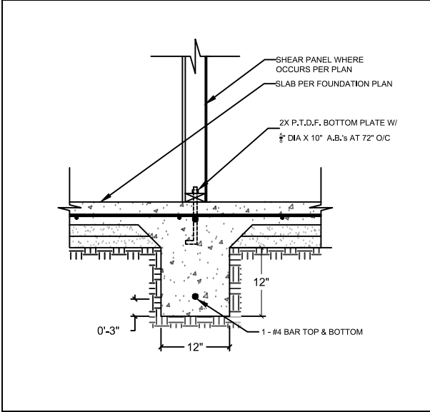
2 INTERIOR FOOTING
