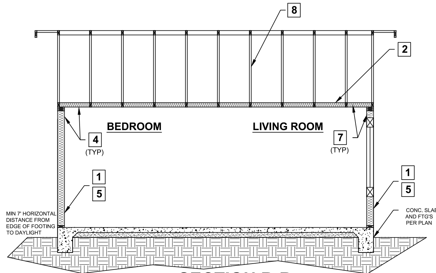
SECTION B-B
