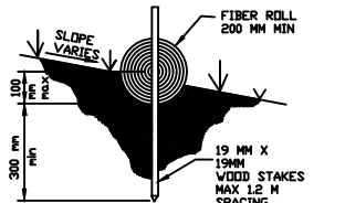
ENTRENCHMENT DETAIL NO SCALE
