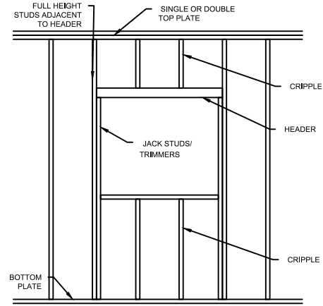
4 TYPICAL FRAMING AT OPENING
