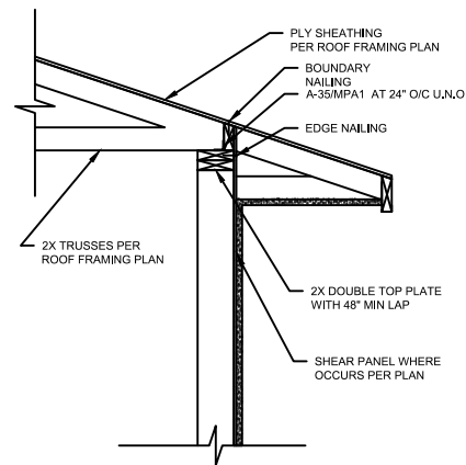
1 EAVE (SHEAR TRANSFER)
