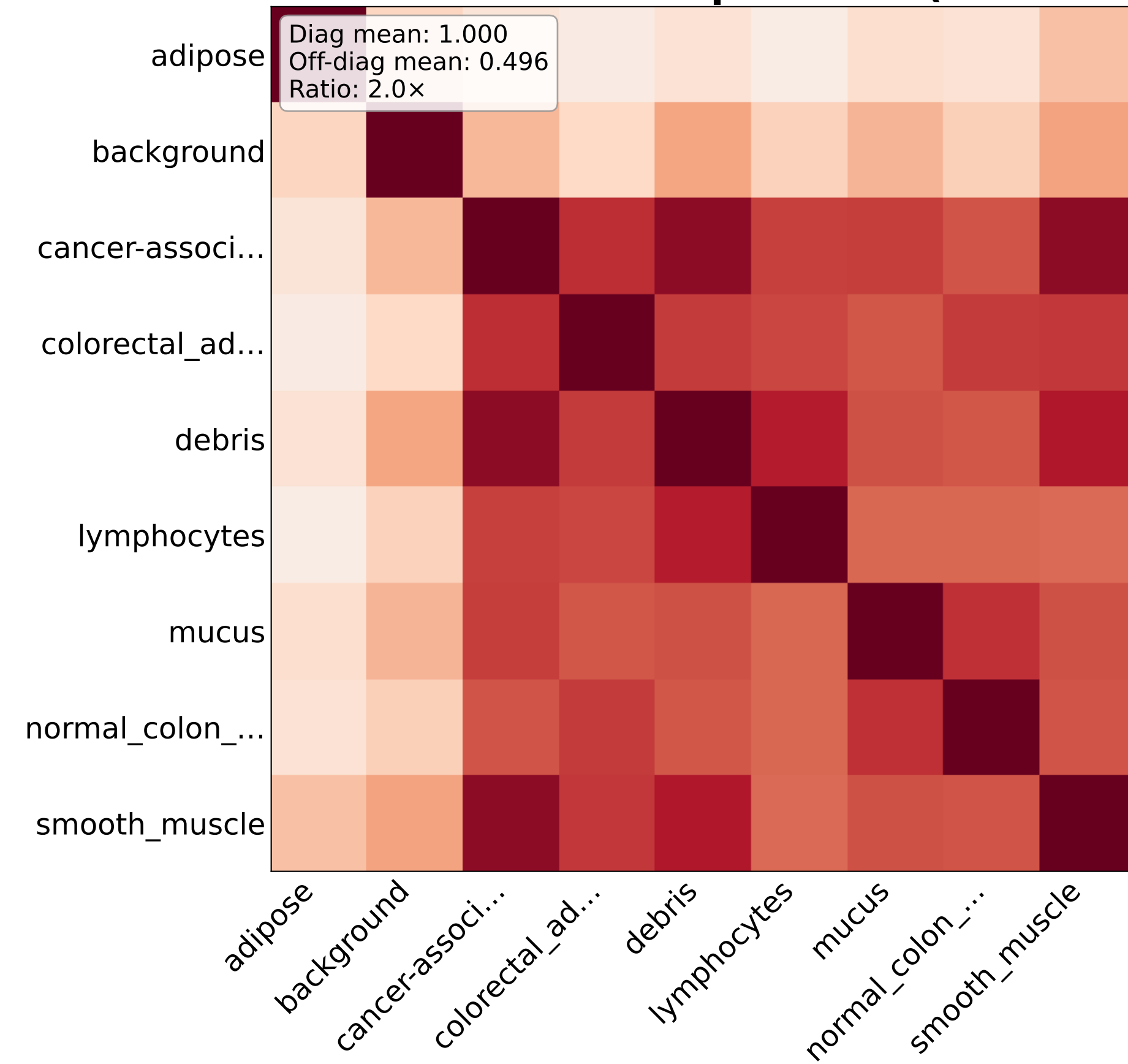
LoRA backbone + Adapted SAE (medmnist)
