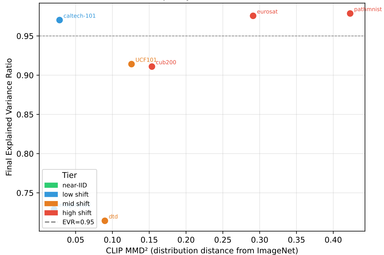
SAE quality vs domain shift
