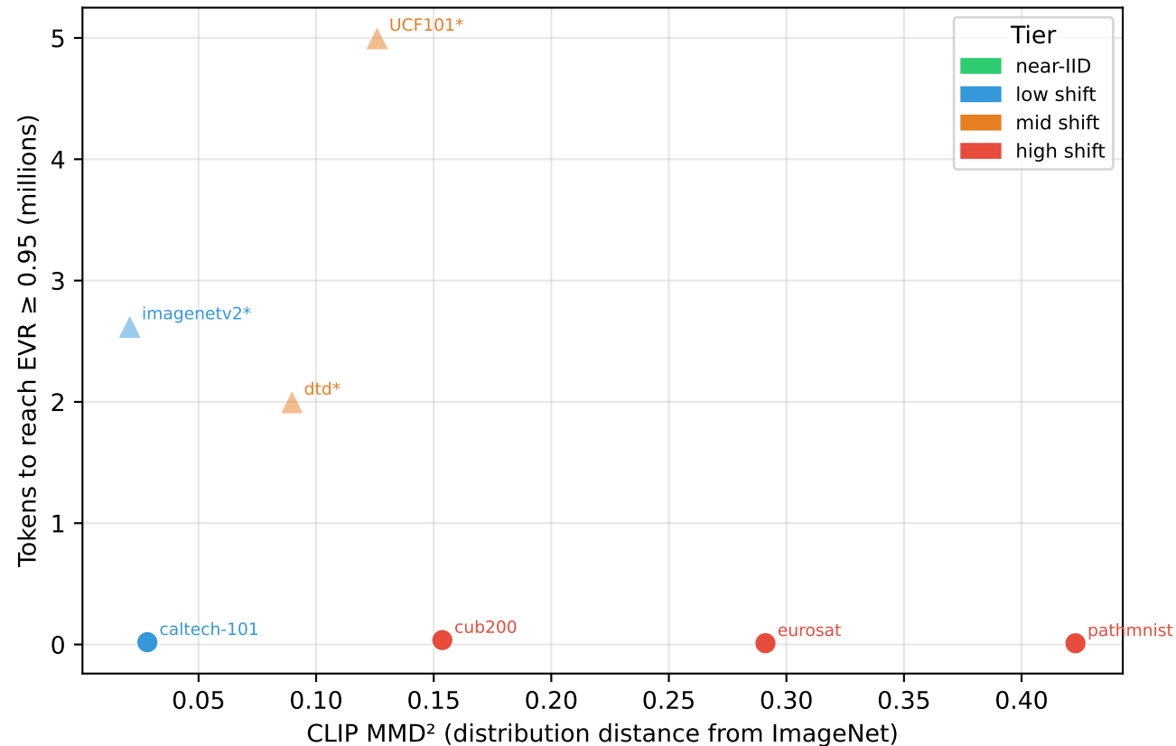
Training effort to convergence (EVR \geq 0.95 ) vs domain shift (^ = never reached threshold)
