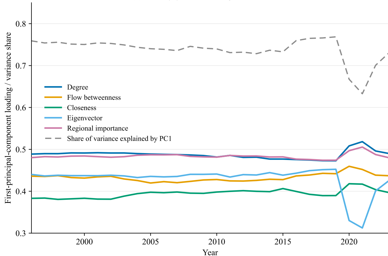
(b) Year-by-year PCA weights, 1996–2023
