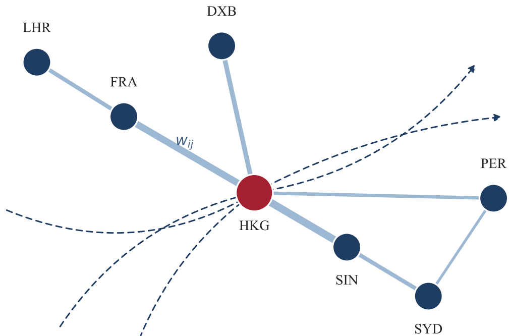
(a) Airport network and link intensities
