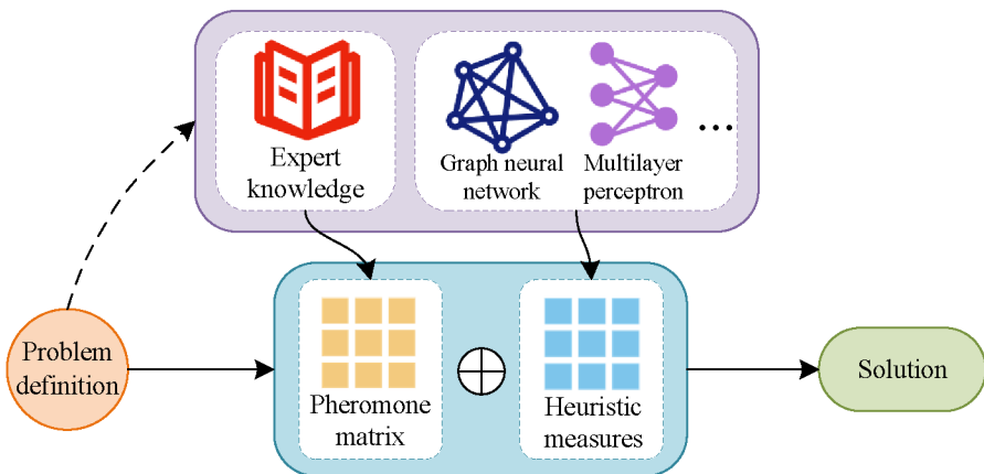
(a) NCO-ACO hybrid methods
