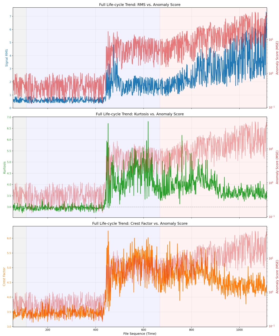
FIGURE 3. Cross-dataset validation on bearing B04. Despite differences in mechanical failure modes, HybridMamba++ maintains high sensitivity to incipient faults, showing co
