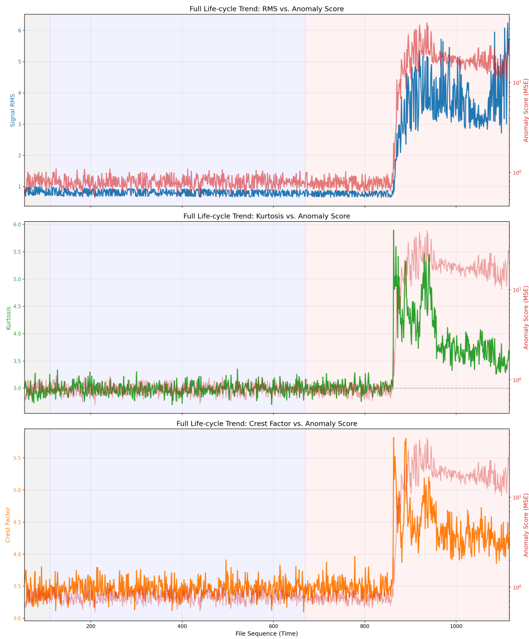
FIGURE 2. Full life-cycle degradation trend for bearing B02. The shaded regions indicate the initial skip period (gray), training/validation area (blue), and the test/fault area (red).
