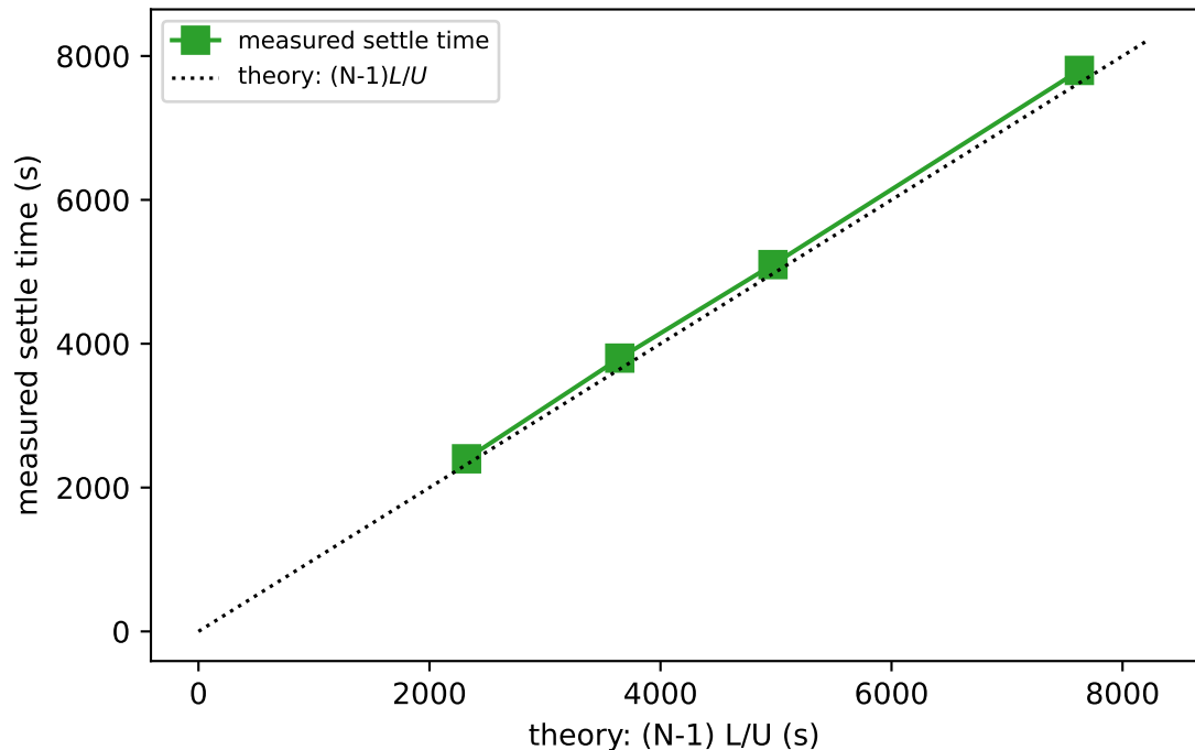
(b) F1 verified: row settles at \approx (N-1)L/U (2-4% error, L/D=10 )
