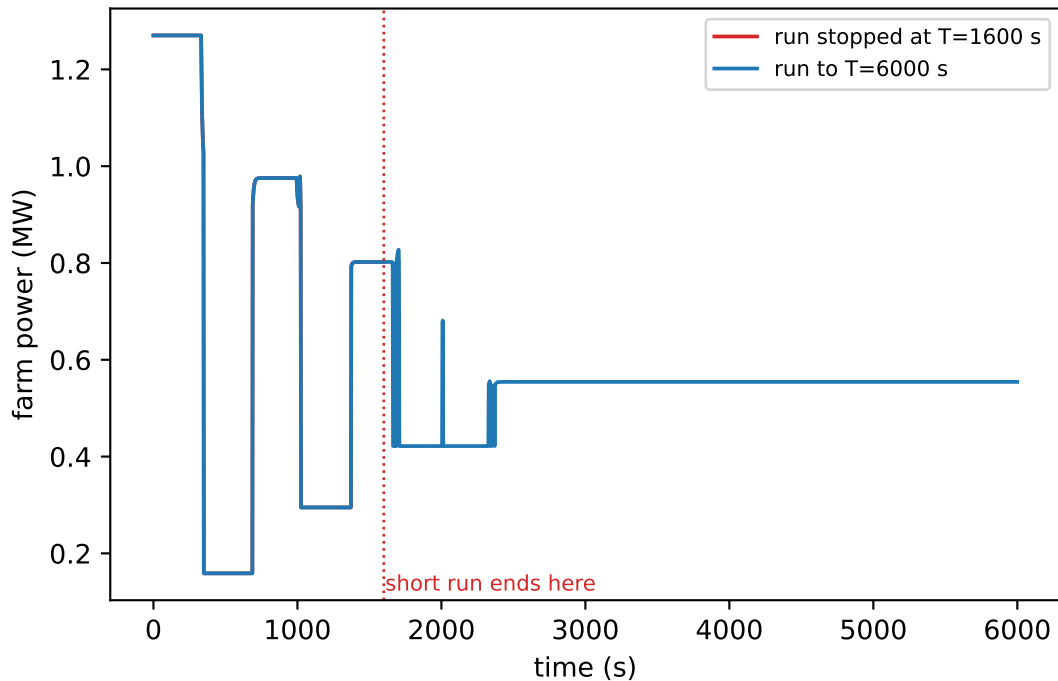
(a) The short-run illusion at L/D=10 : the 1600 s run averages +13% higher than the settled state
