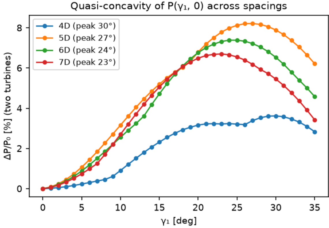
Figure 12: Two-turbine P(\gamma_1, 0) is quasi-concave with a single peak in the valid region for every spacing (4D–7D); the 4D tail beyond 25^\circ lies in the excluded boundary zone.
