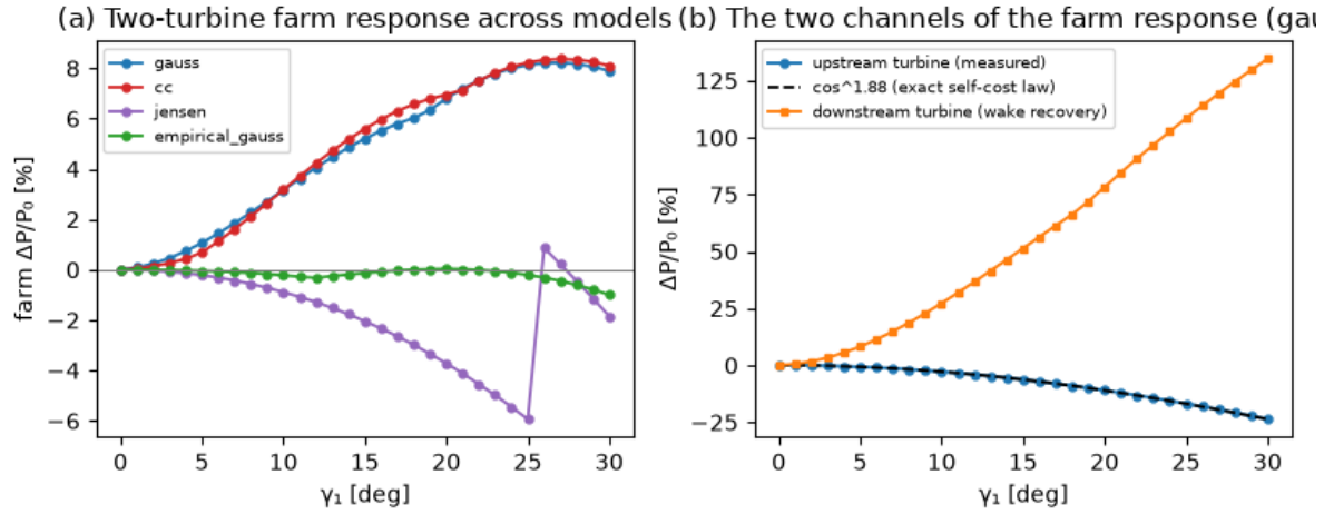
Figure 7: (a) Two-turbine farm response across four FLORIS model families; (b) the farm response decomposes into the exact \cos^{1.88} self-cost term of the upstream turbine and the rising wake-recovery term of the downstream turbine.
