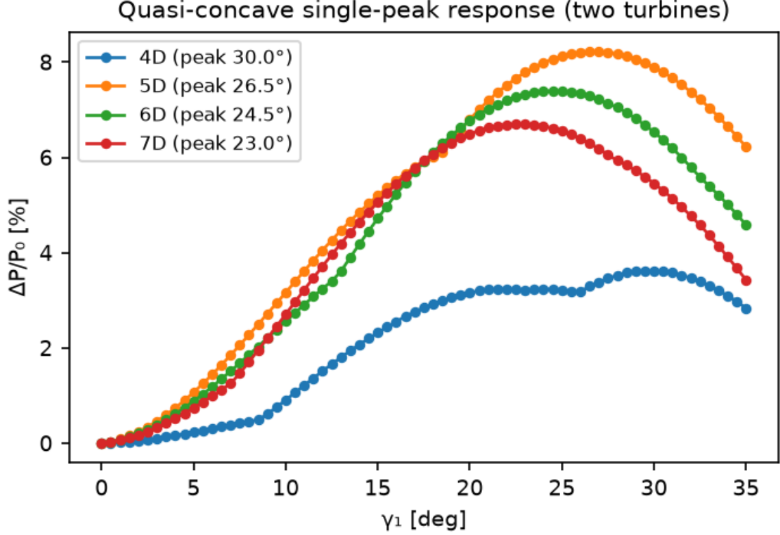
Figure 2: Two-turbine P(\gamma_1, 0) is single-peaked for every spacing ( 0.5^\circ grid): peaks at 30^\circ (4D, boundary of the warning zone) / 26.5^\circ (5D) / 24.5^\circ (6D) / 23^\circ (7D); both branches monotone for 5D–7D, the 4D tail beyond 25^\circ excluded (negative-velocity warnings).
