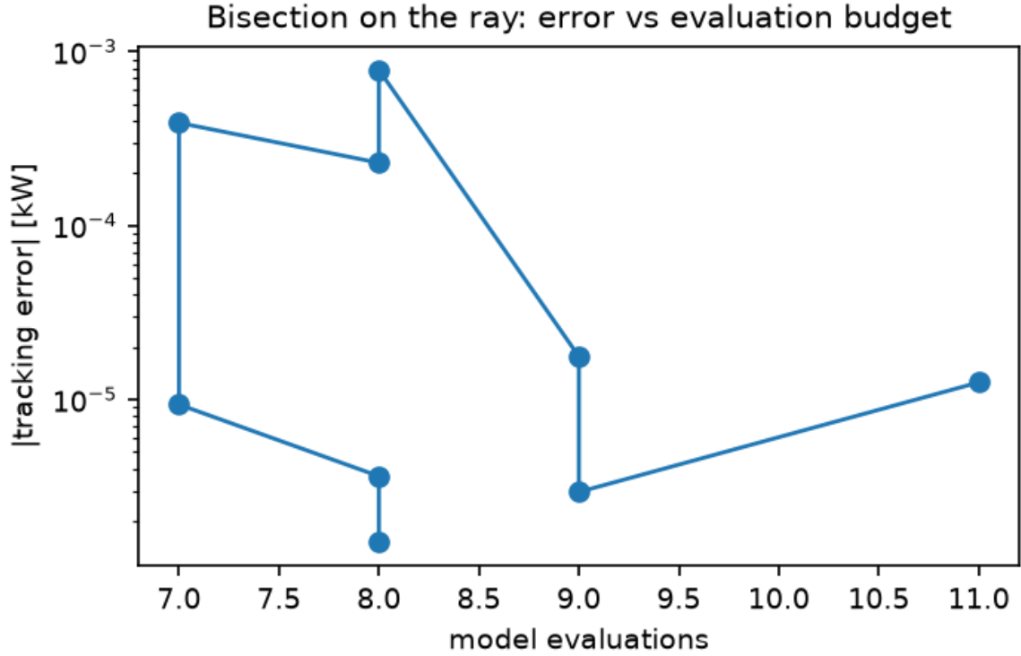
Figure 3: Bisection on the ray: |\text{tracking error}| versus model evaluations across the nine targets of Table 1. Every target is reached in 7–11 evaluations; the error floor ( \leq 7.8 \cdot 10^{-4} kW) is the solver tolerance, not the method.
