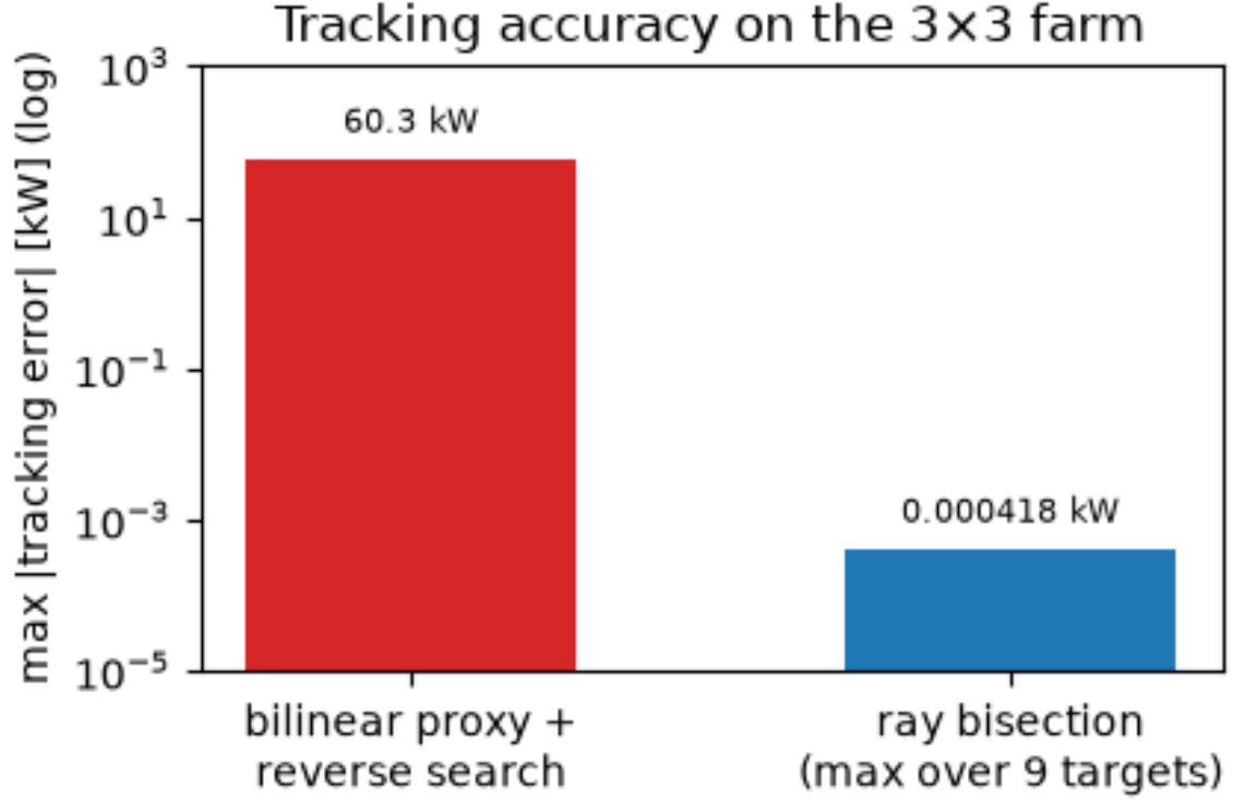
Figure 4: Proxy versus exact inverse on the 3 \times 3 power range: the bilinear-proxy reverse search errs by up to 60.28 kW (0.60 % of P_{\max} ); ray-bisection at a comparable budget (7–11 calls) reaches \leq 7.8 \cdot 10^{-4} kW, five orders of magnitude better.
