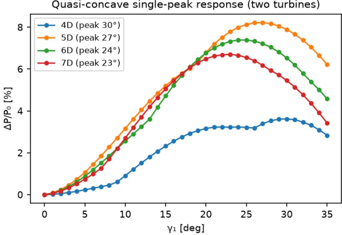
Figure 2: Two-turbine P(\gamma_1, 0) is quasi-concave with a single peak for every spacing (4D–7D): peaks at 30^\circ (4D, boundary) / 27^\circ (5D) / 24^\circ (6D) / 23^\circ (7D), both branches monotone within the validity region \gamma_1 \leq 25^\circ .
