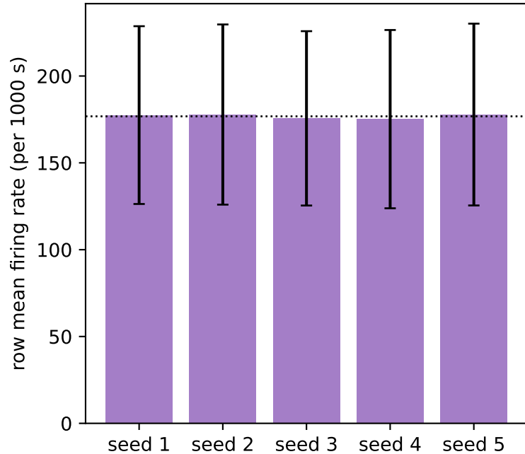
(a) Firing rate: 175-178/1000 s across 5 seeds ( \pm 1\% )
