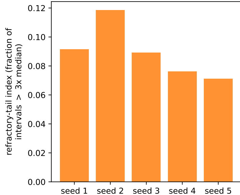
(c) Refractory-tail index stable (7-12% across seeds)
