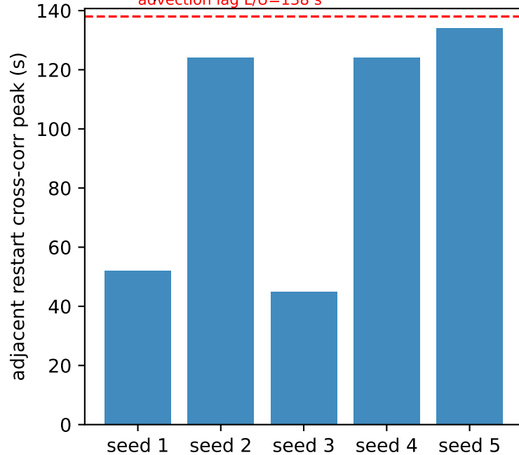
(b) Correlation peak wanders between atmospheric ( \sim 50 s) and advection ( \sim 130 s) advection lag L/U = 138 s
