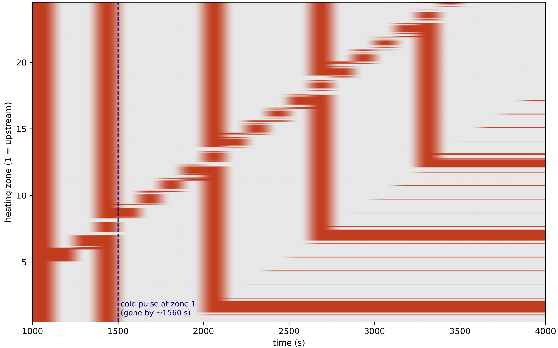
Thermostatic heater chain: a local cold pulse launches a regenerative heater-firing wave downstream (red = heater on), at the fluid speed
