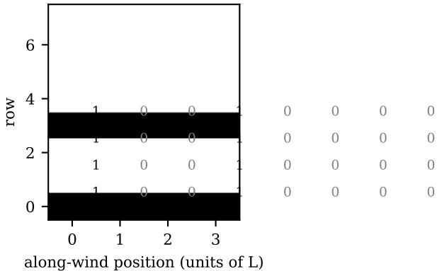
(a) settled 2-D state ( 4 \times 8 , L_r=3D )
