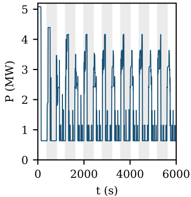
(b) wind reversals every 400 s drive reconfigu
