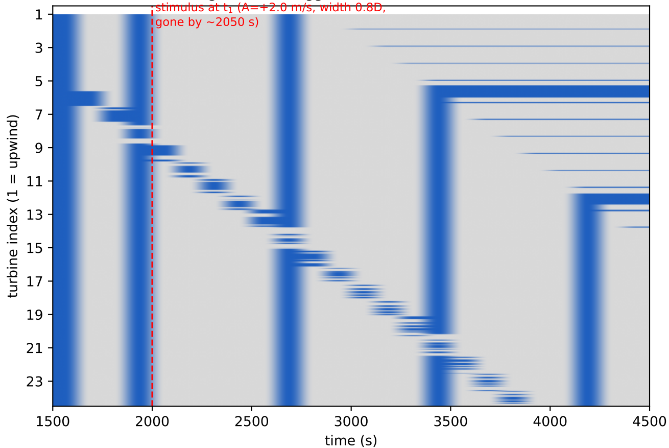
(a) Regenerative trigger wave (blue = above cut-in)
