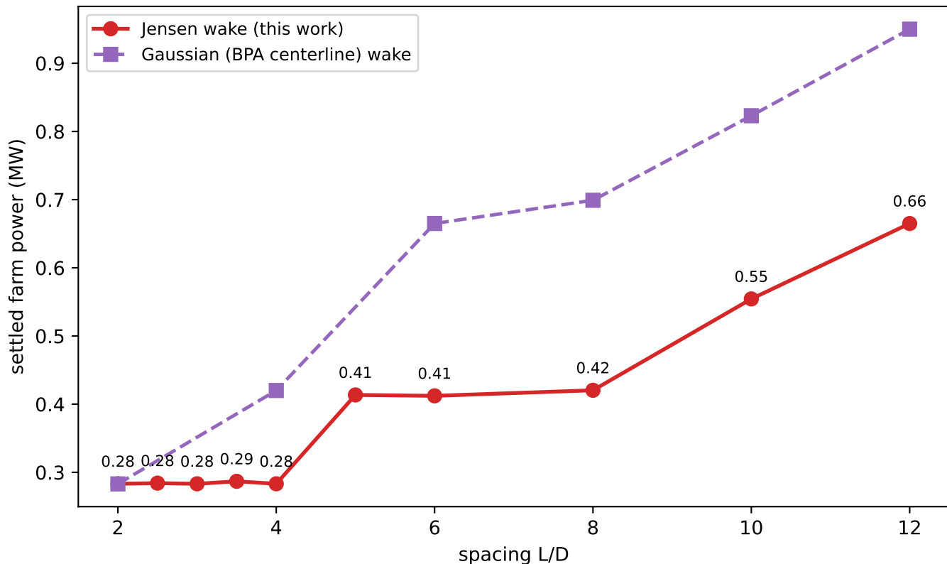
Quantized power steps: staircase vs spacing ( N=8 , U_0=3.8 m/s, T=6000 s, settled; two wake kernels)
