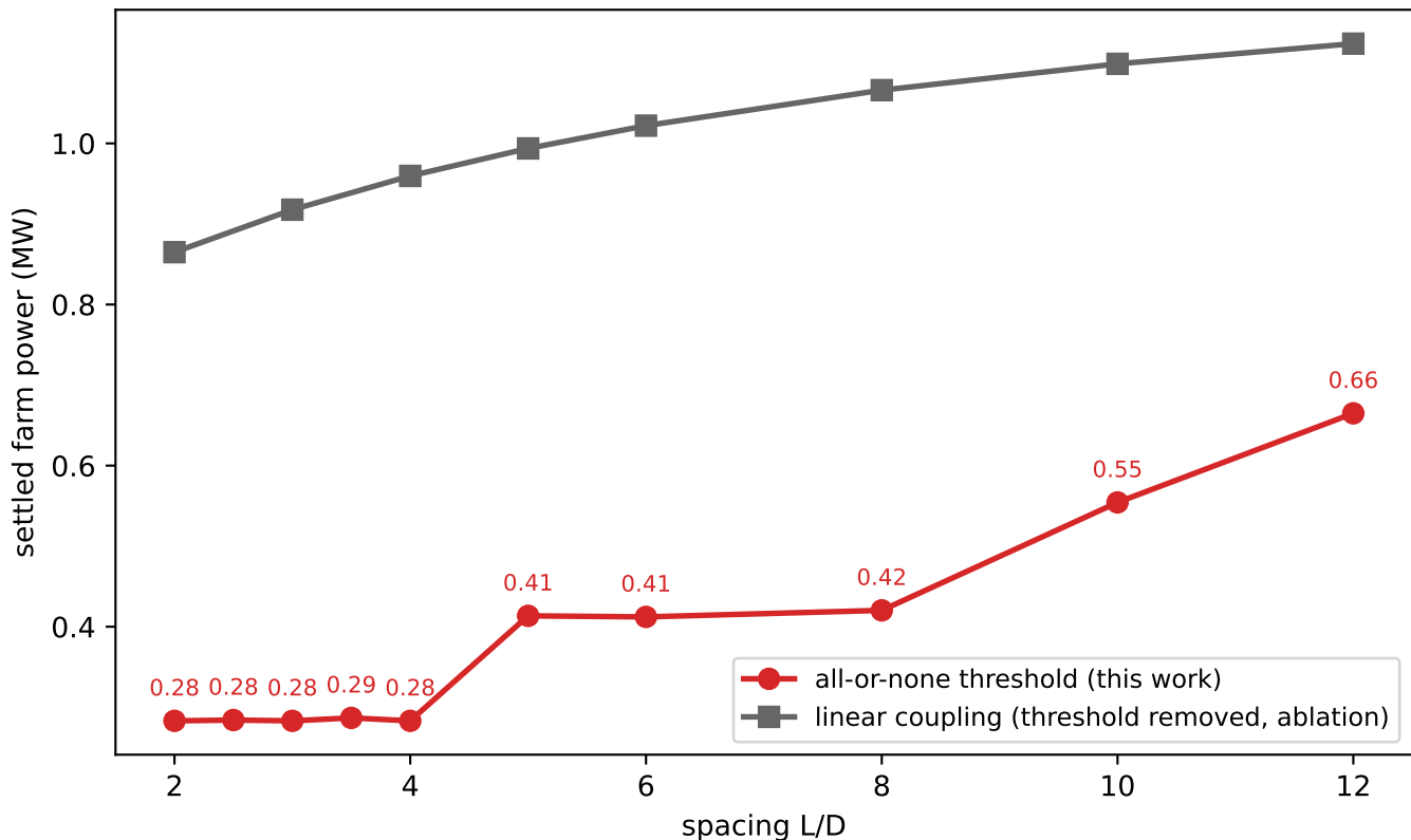
Ablation: removing the cut-in threshold removes the staircase (threshold row: discrete steps; linear row: smooth monotone, all machines spinning)
