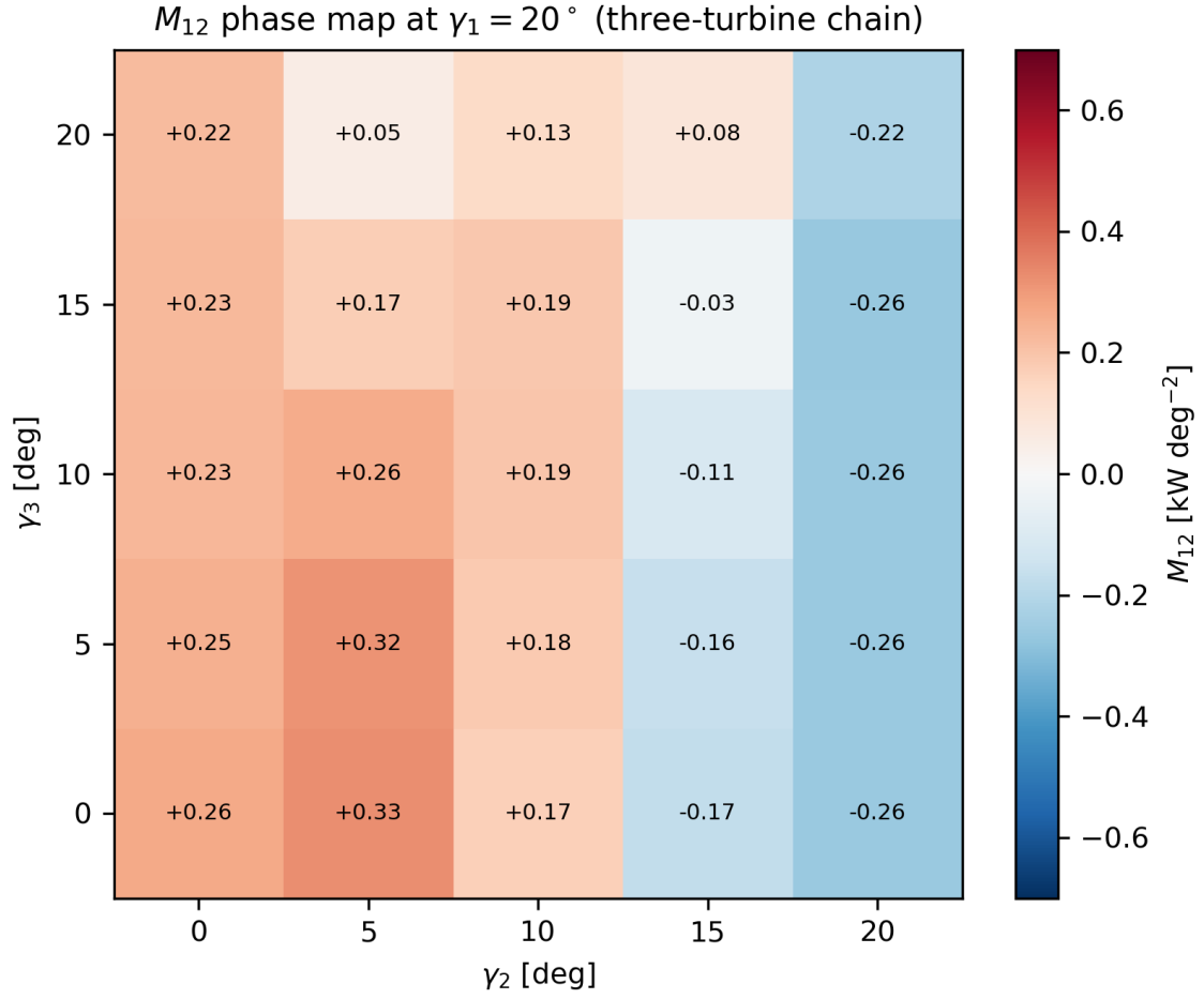
Figure 1: The phase boundary of the chain pair on the reported 0–20° grid: M_{12} is positive (complementarity, warm colours) at small \gamma_2 and flips negative (substitution, cool colours) as (\gamma_2, \gamma_3) move right, because the shared-beneficiary channel through turbine 3 strengthens with \gamma_3 . Operating-point corners at \gamma \geq 25^\circ are excluded as a model-validity boundary.
