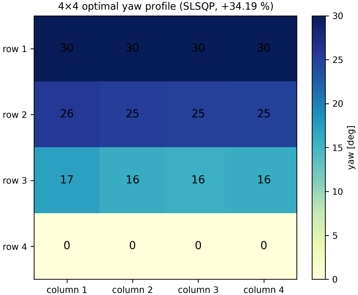
Figure 6: The 4 \times 4 optimum is row-synchronous and monotonically decreasing downstream: [30, 30, 30, 30] , [25.8, 25.2, 25.1, 25] , [17.2, 16, 15.7, 16] , [0, 0, 0, 0] degrees (+34.19 %).
