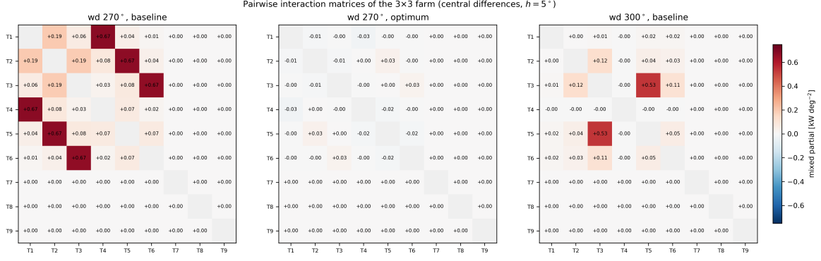
Figure 2: Pairwise mixed partials make the wake DAG quantitative: chain pairs carry the largest entries at the origin, lateral pairs are weaker complements, the last row is decoupled, and the pattern re-assembles around the rotated flow at 300^\circ . Diagonal entries are omitted to isolate pairwise interactions.
