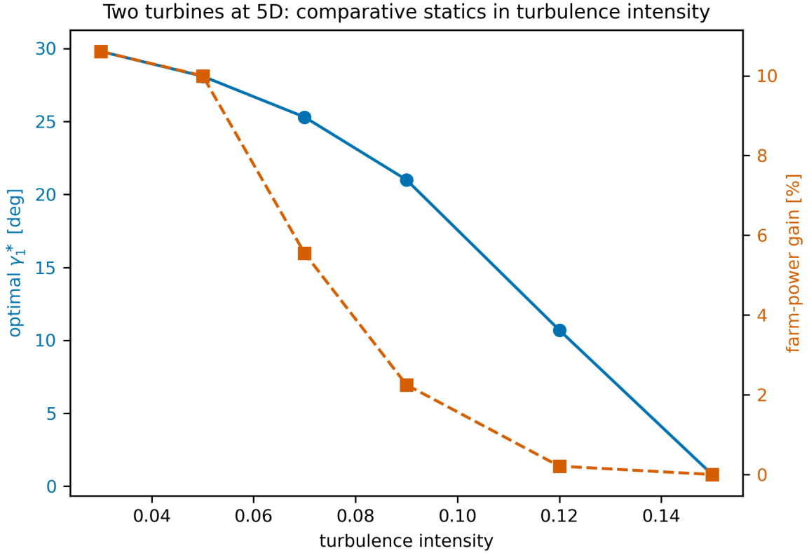
Figure 5: Comparative statics: the optimal yaw \gamma_1^* decreases monotonically from 29.8^\circ to 0.8^\circ as TI rises 0.03 \rightarrow 0.15 , exactly as the single-crossing argument predicts, with no convexity assumption.
