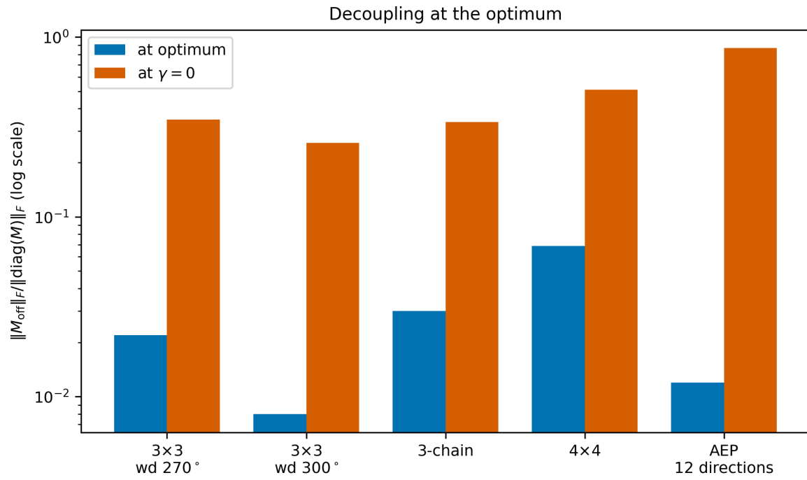
Figure 3: The decoupling law: at power-maximizing profiles the off-diagonal-to-diagonal Hessian ratio falls by an order of magnitude (0.35 to 0.02 on the 3 \times 3 farm).
