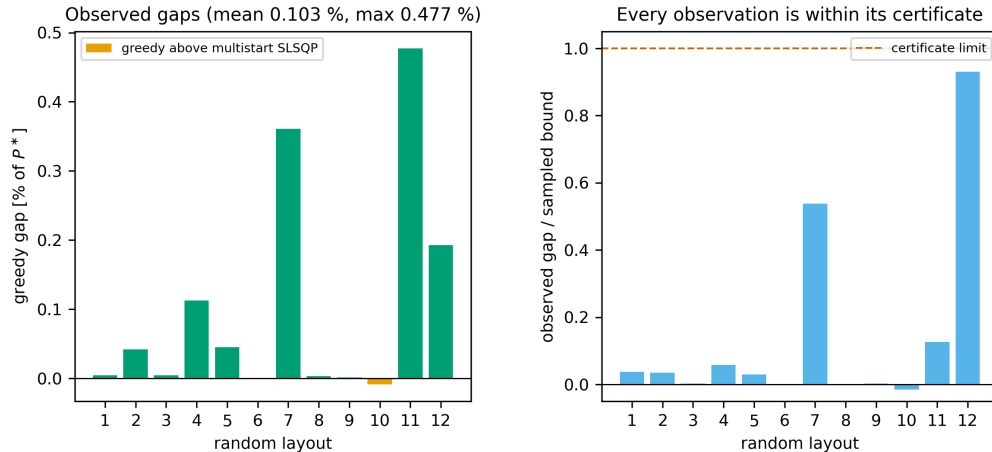
Figure 4: Greedy near-optimality and the bounded-interaction certificate on 12 random layouts. Left: measured gaps (mean 0.103 %, max 0.477 %). Right: each observed gap divided by its sampled interaction-energy bound; every ratio is at most one.
