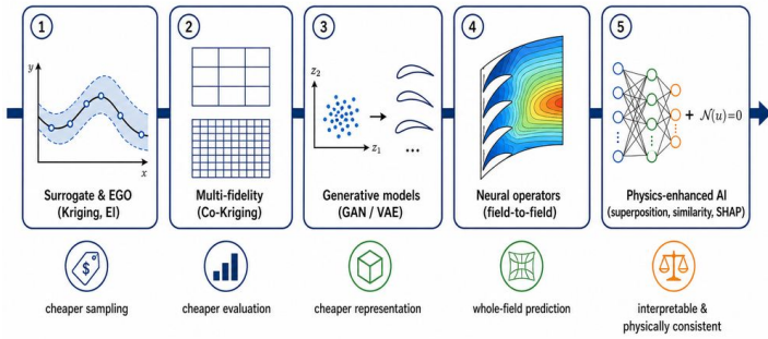
AI4Turbomachinery evolution map (English labels; this lecture is stage 3: generative model)
