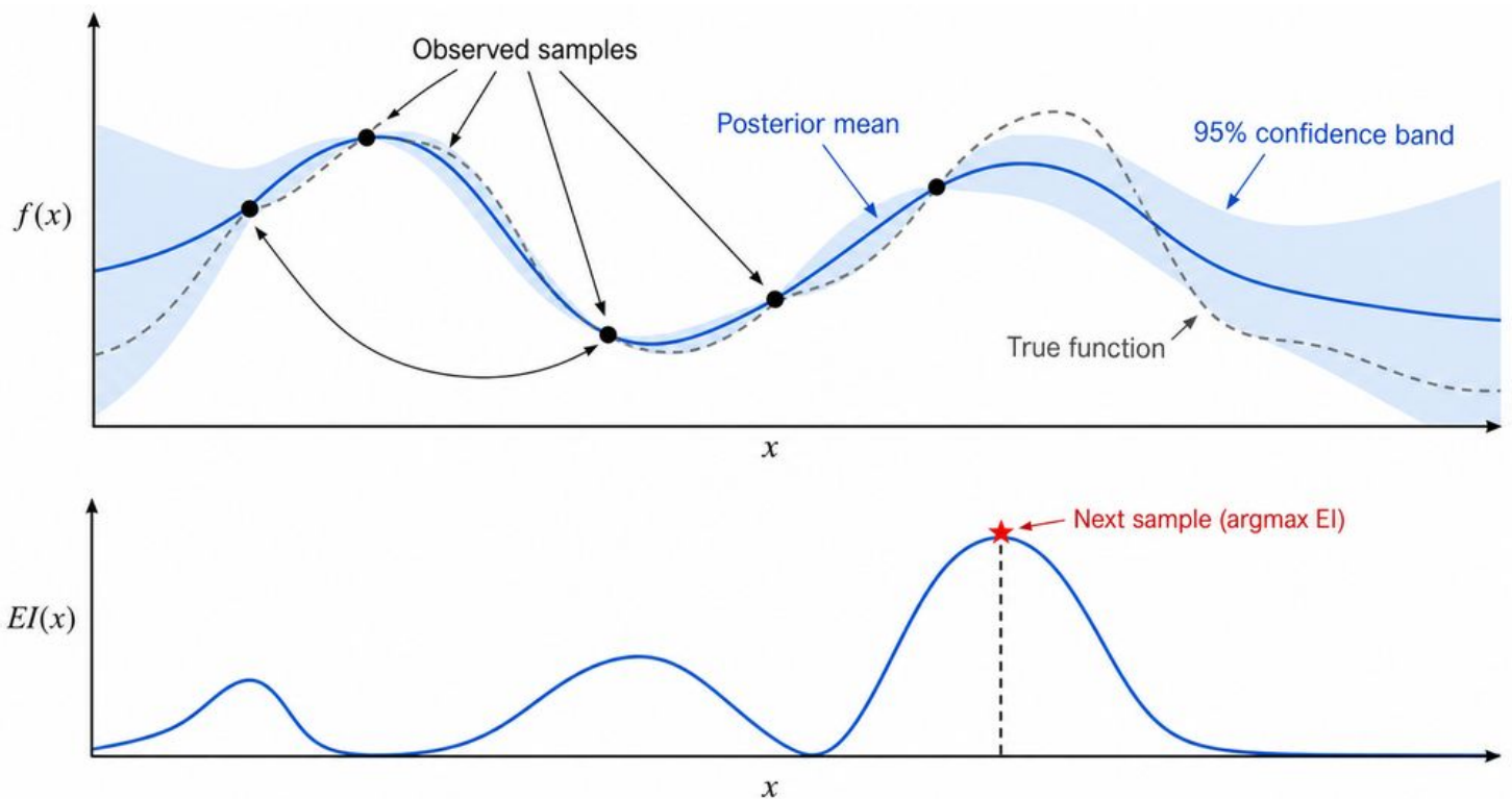
gaussian process and acquisition function (English labels; counterpart)
