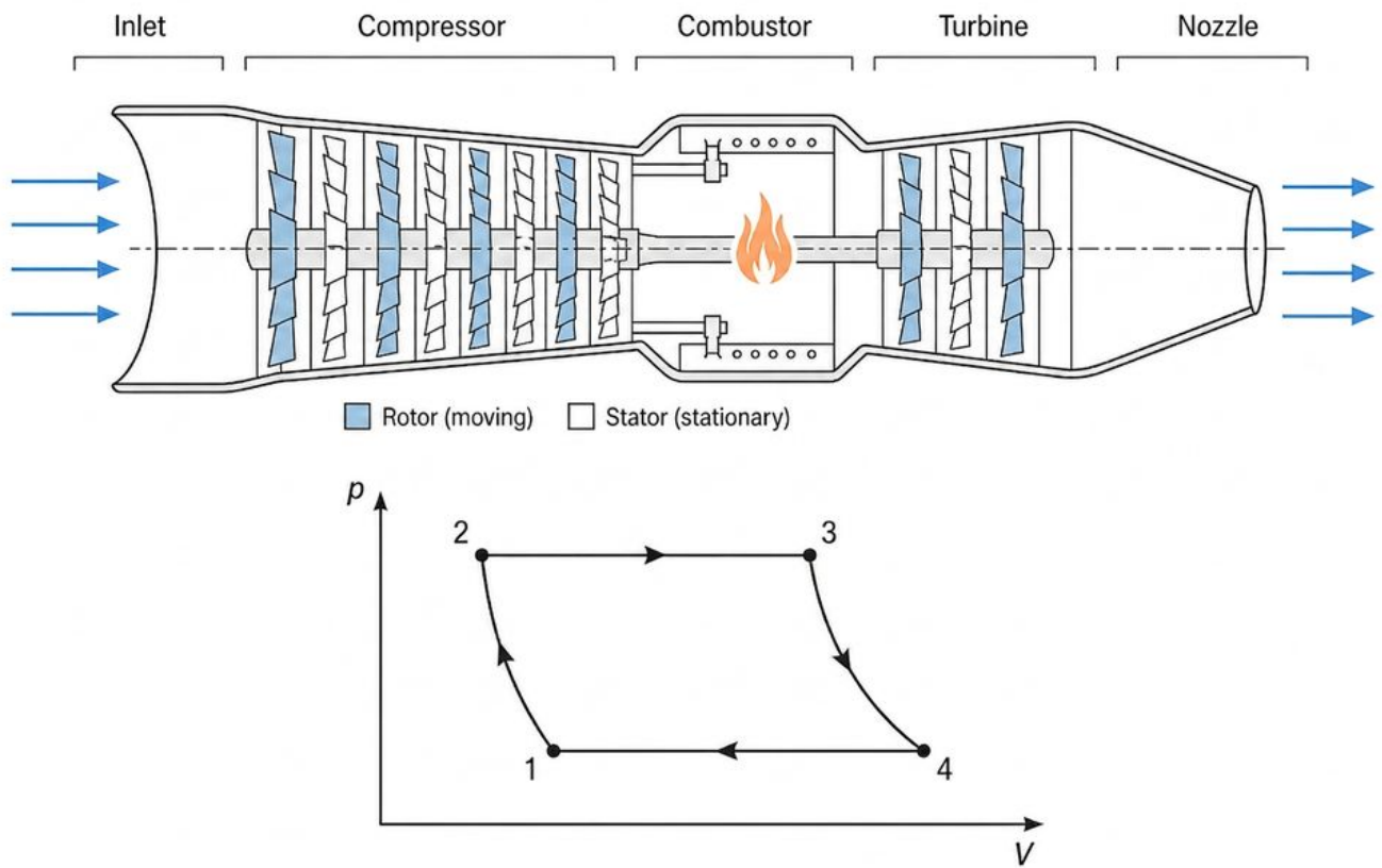
gas turbine working principle (English labels; chapter0 counterpart)
